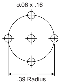
PCB Pattern
