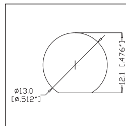
AC-BNC-PJA-75 AC-BNC-JJA-75
