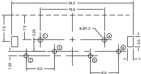
Recommended PCB Layout (Bottom View)
