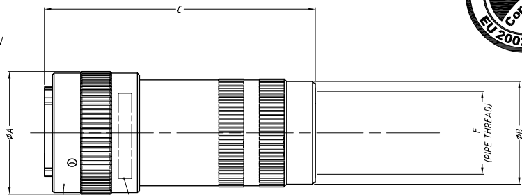
CONTACTS NOT SHOWN REFER TO TABLE FOR No OF CONTACTS
