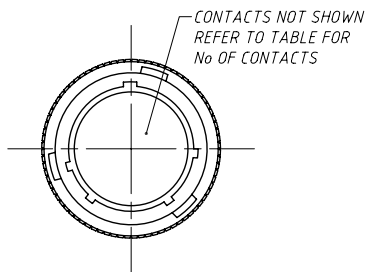
STRAIGHT PLUG 62IN SERIES WITH GOLD PLATED SOLDER PIN CONTACTS
