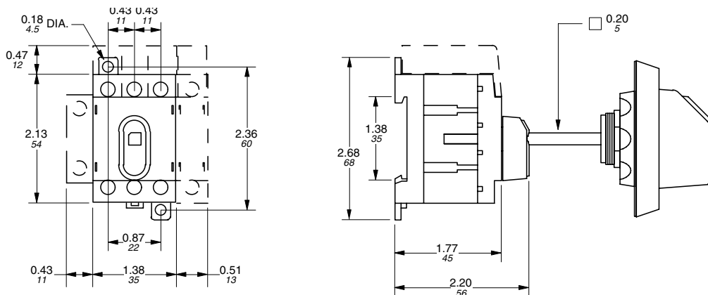
CDNF16, CDNF25, CDNF32 — base & DIN rail mounted switch
