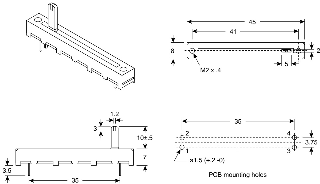
Dimensions (mm)
