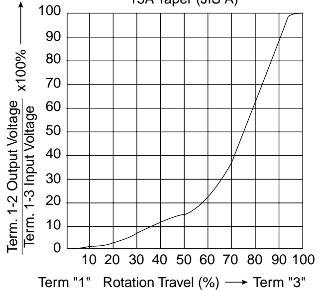
Standard Resistance Taper 15A Taper (JIS A)
