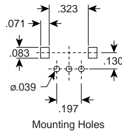
Mounting Holes
