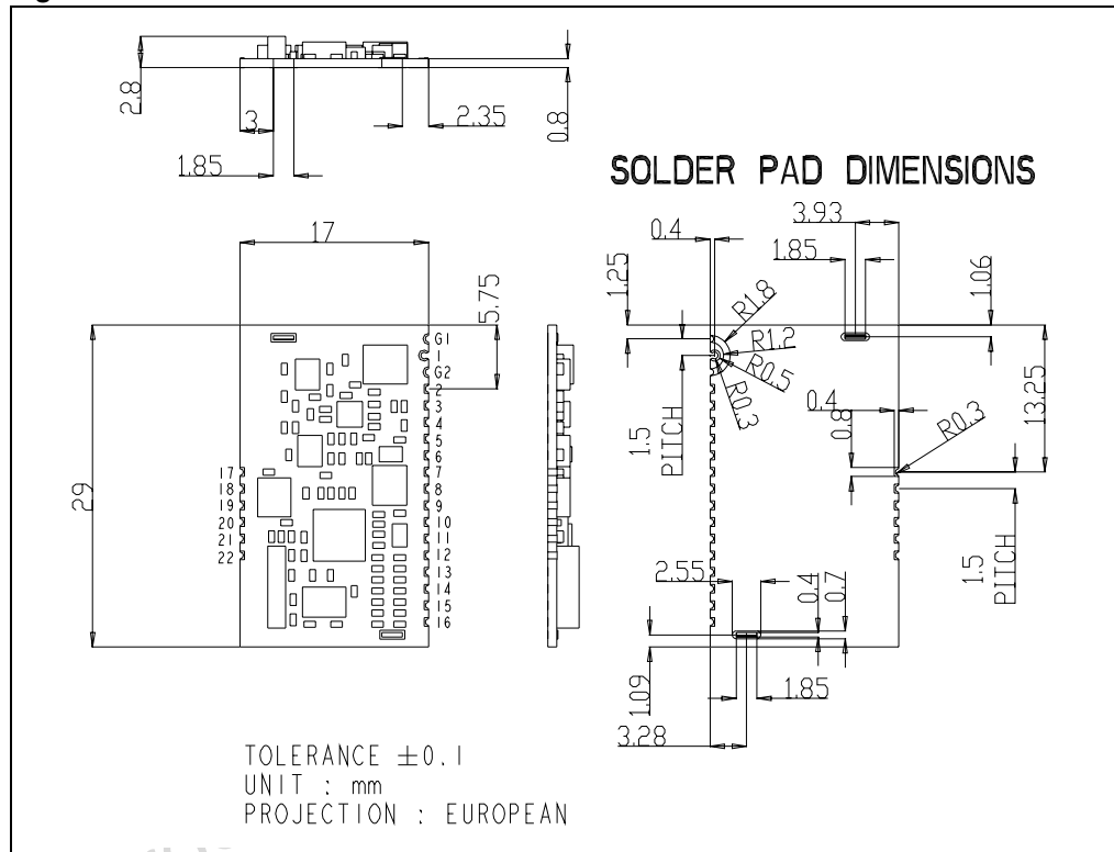
Figure 2. Mechanical dimensions
