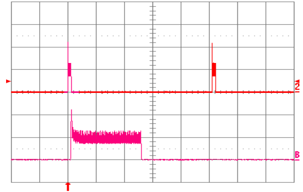
Fig. 18: Load current (top trace, 5 A/div., 20 ms/div.) into a 10 m \Omega short circuit during restart, at V_{in} = 24 V. Bottom trace (5 A/div., 1 ms/div.) is an expansion of the on-time portion of the top trace.
