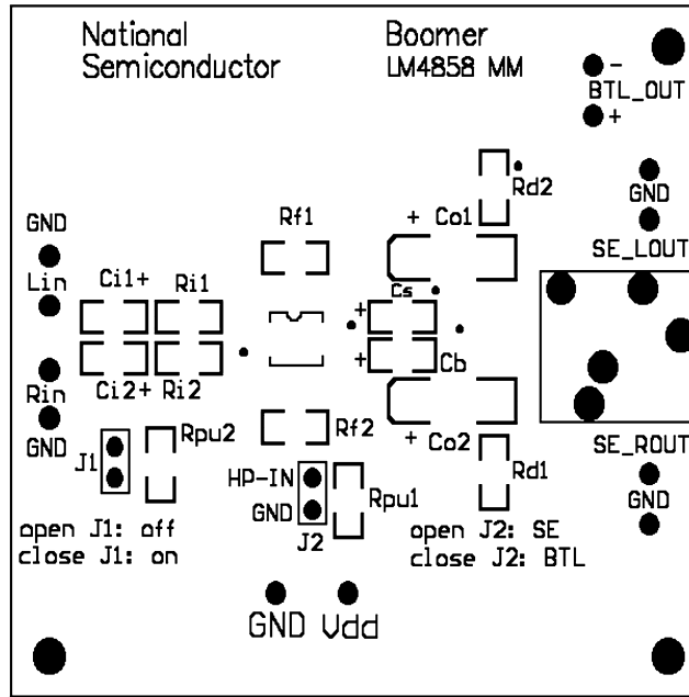
FIGURE 2. Recommended MM PC Board Layout: Component-Side SilkScreen
