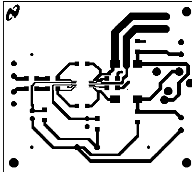
FIGURE 3. Recommended MM PC Board Layout: Component-Side Layout
