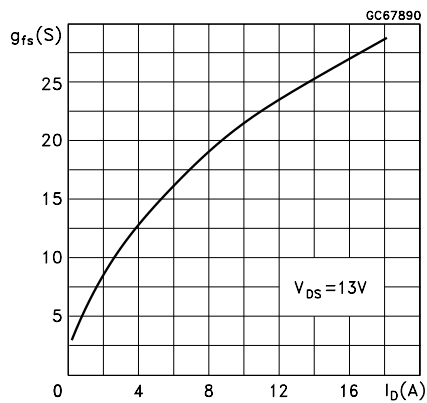
Transconductance
