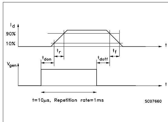
Fig. 6: Waveforms
