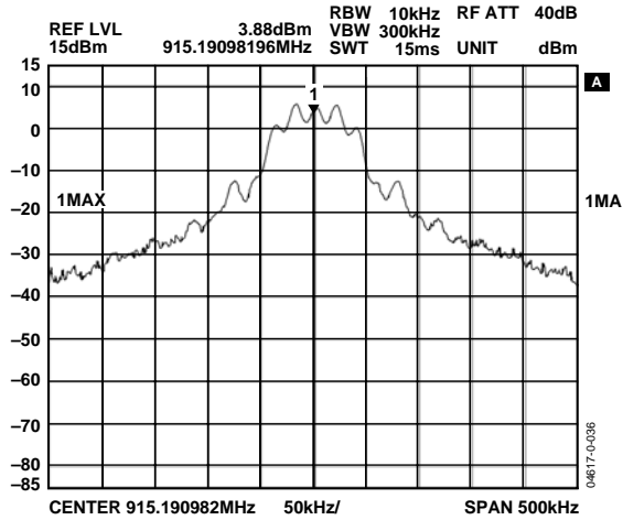
Figure 22. FSK Modulation, \text{Power} = 10 \text{ dBm} , \text{Data Rate} = 38.4 \text{ kbps} , F_{\text{deviation}} = \pm 19.2 \text{ kHz}
