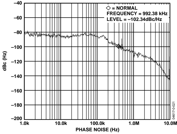
Figure 21. Phase Noise Response— I_{CP} = 1.44 \text{ mA} , I_{VCO} = 3.0 \text{ mA} , R_{FOUT} = 915.2 \text{ MHz} , PFD = 10 \text{ MHz} , \text{Power} = 10 \text{ dBm} , \text{PA Bias} = 5.5 \text{ mA}
