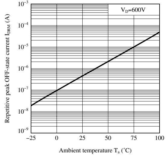
Fig.7-b Repetitive Peak OFF-state Current vs. Ambient Temperature (S202T01)
