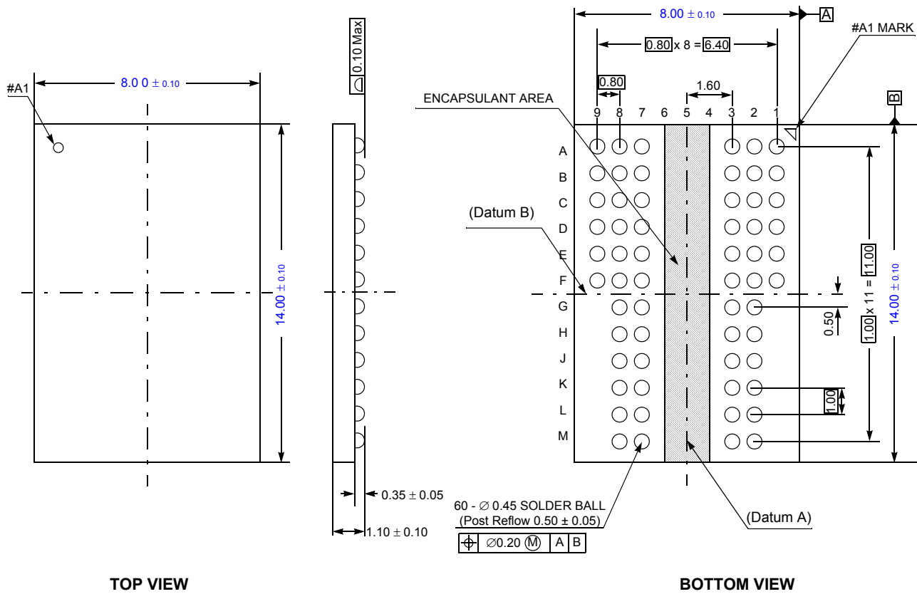
60Ball FBGA 256Mb Package Dimension
