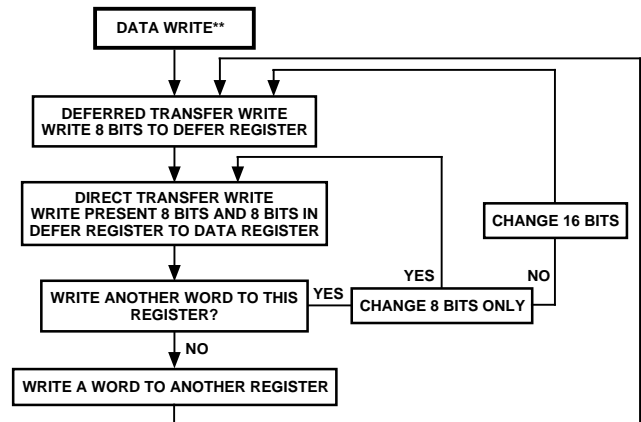
Figure 24. Data Writes
