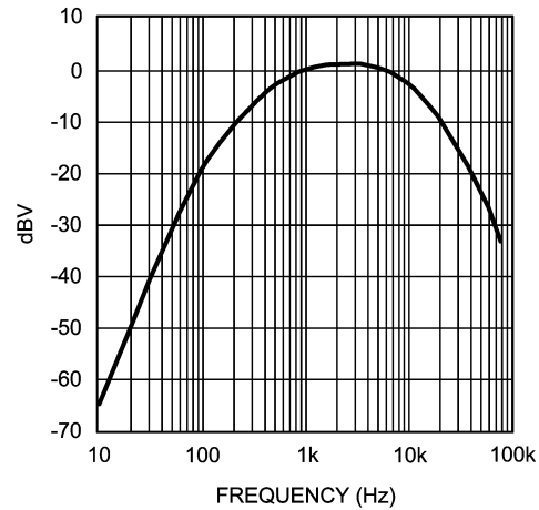
FIGURE 2. A-Weighted Filter
