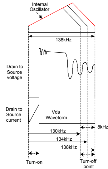
Figure 14. Frequency Modulation Waveforms
