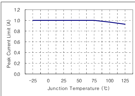
Peak Current Limit vs. Temp
