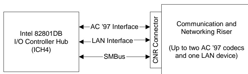
Figure 7. ICH4 and CNR Signal Interface
