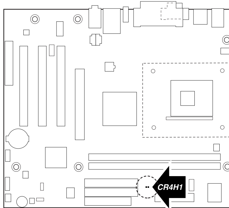
Figure 9. Location of the Standby Power Indicator LED
