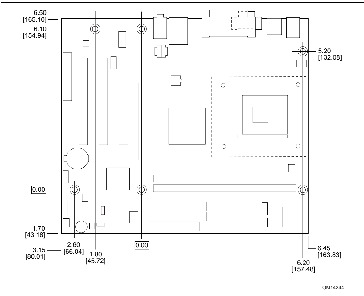
Figure 18. Desktop Board D845EPT2 Dimensions
