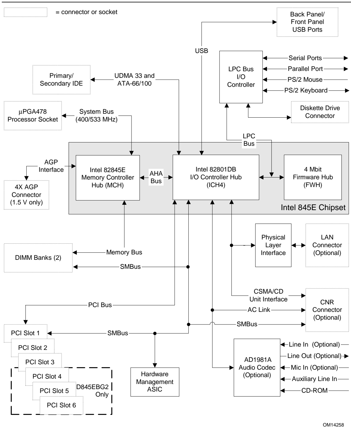
Figure 3. Block Diagram
