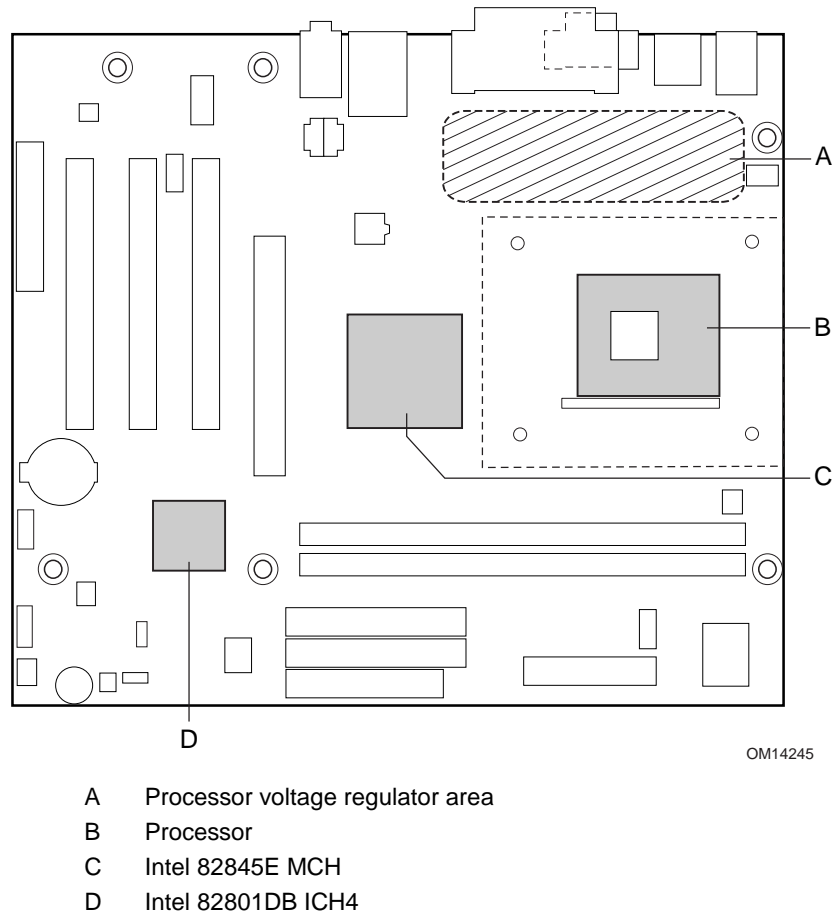
Figure 21. Localized High Temperature Zones
