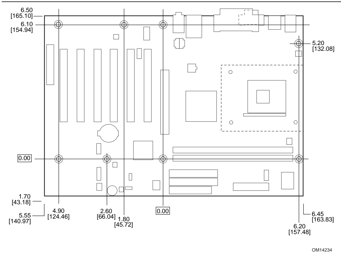
Figure 17. Desktop Board D845EBG2 Dimensions
