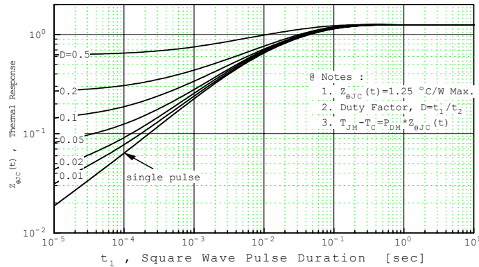
Figure 11. Thermal Response
