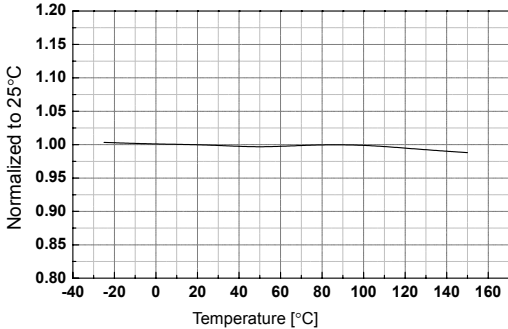
Vcc Start Threshold Voltage vs. Temp.
