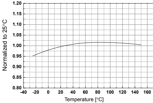
Operating Frequency vs. Temp.
