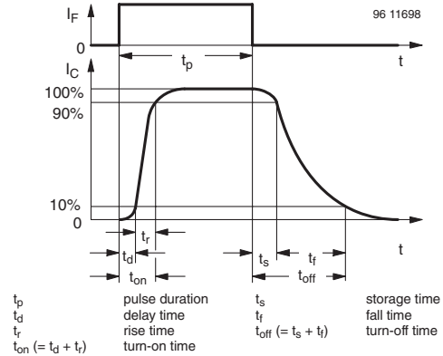
Figure 2. Switching Times
