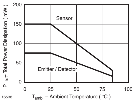
Figure 3. Derating diagram
