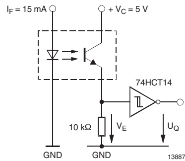
Figure 12. Application example
