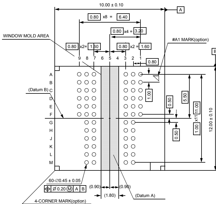
Bottom view
