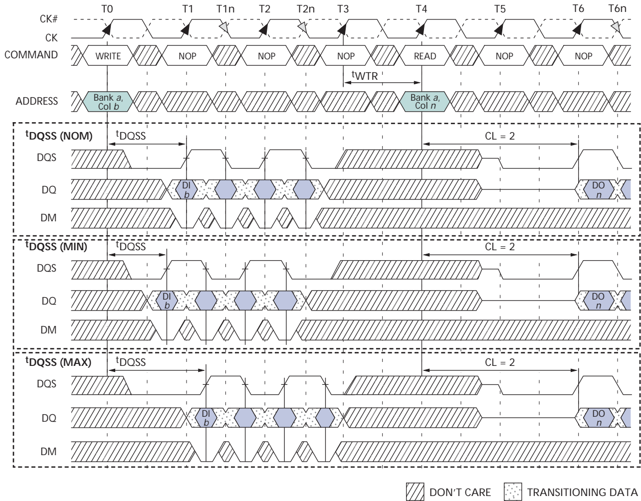
Figure 40: WRITE-to-READ – Uninterrupting
