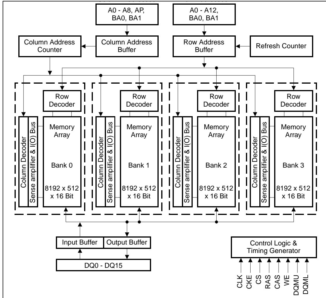
Block Diagram for 16M x16 SDRAM ( 13 / 9 / 2 addressing)
