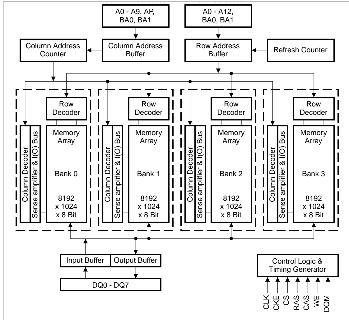
Block Diagram for 32M x 8 SDRAM (13 / 10 / 2 addressing)
