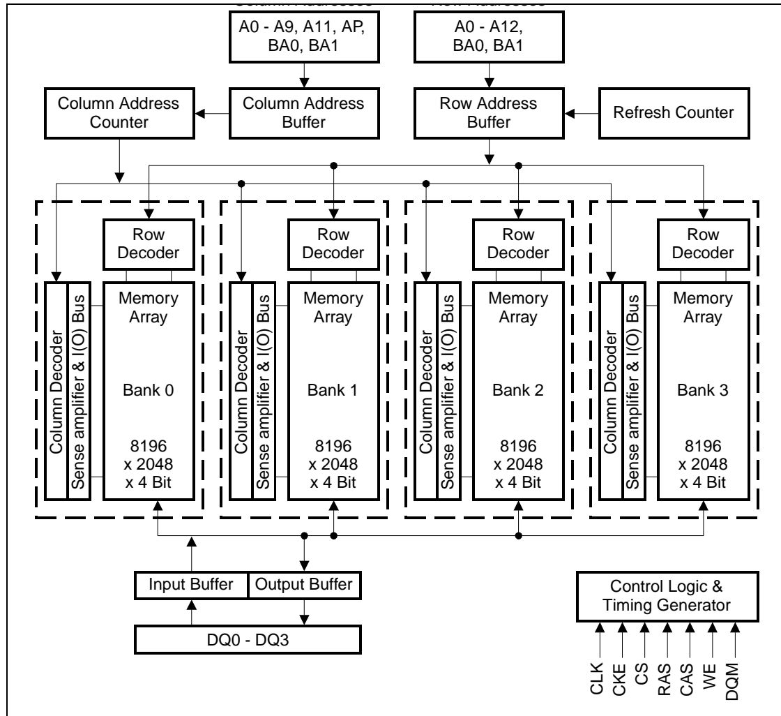
Block Diagram for 64M x 4 SDRAM (13/11/2 addressing)
