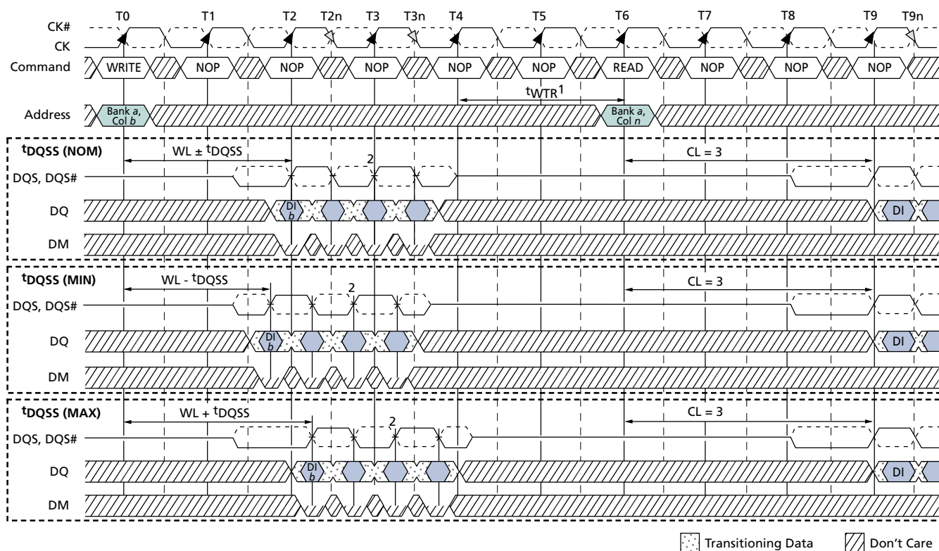
Figure 61: WRITE-to-READ
