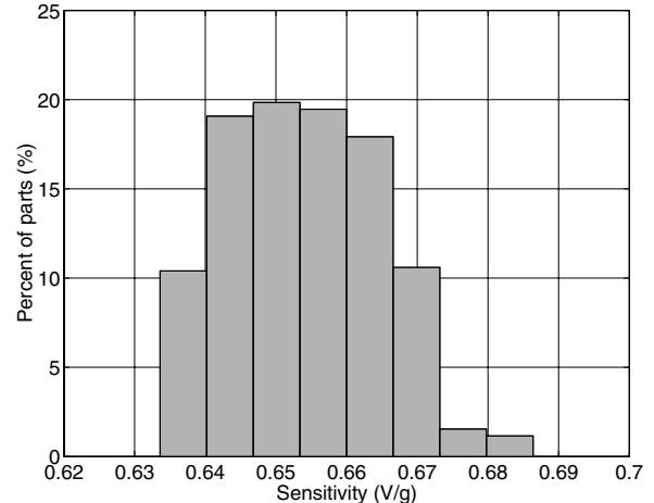
Figure 11. Z axis Sensitivity at 3.3V
