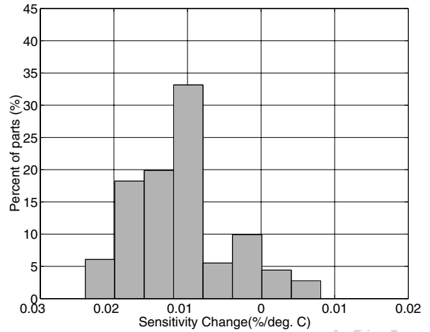
Figure 16. Y axis Sensitivity Change Vs. Temperature
