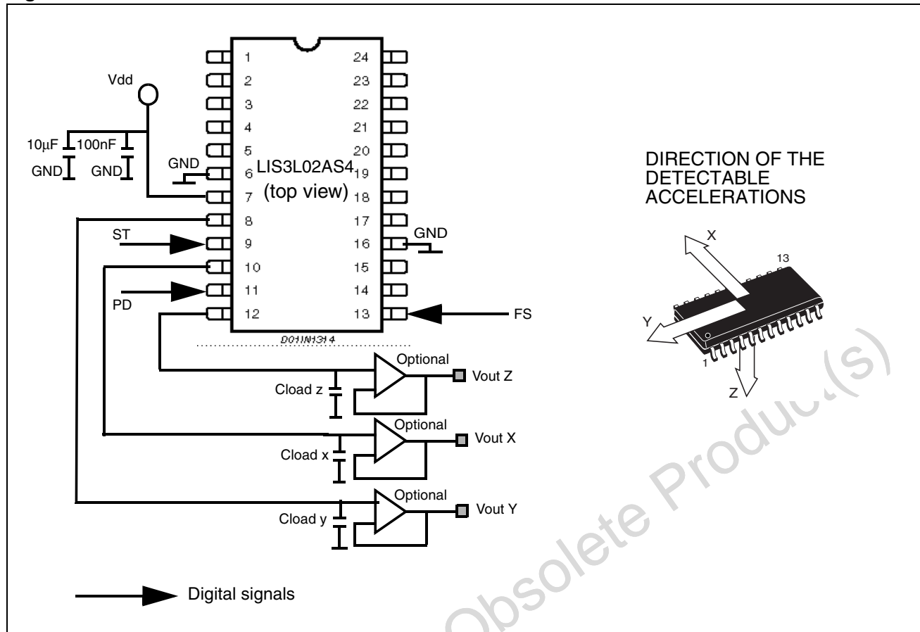
Figure 4. LIS3L02AS4 Electrical Connection
