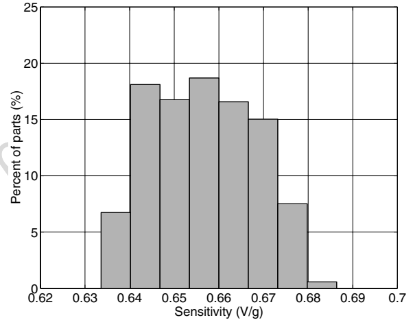
Figure 11. Z axis Sensitivity at 3.3V
