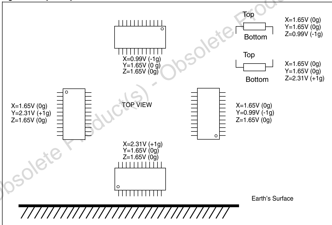
Figure 5 refers to LIS3L02AS4 device powered at 3.3V
