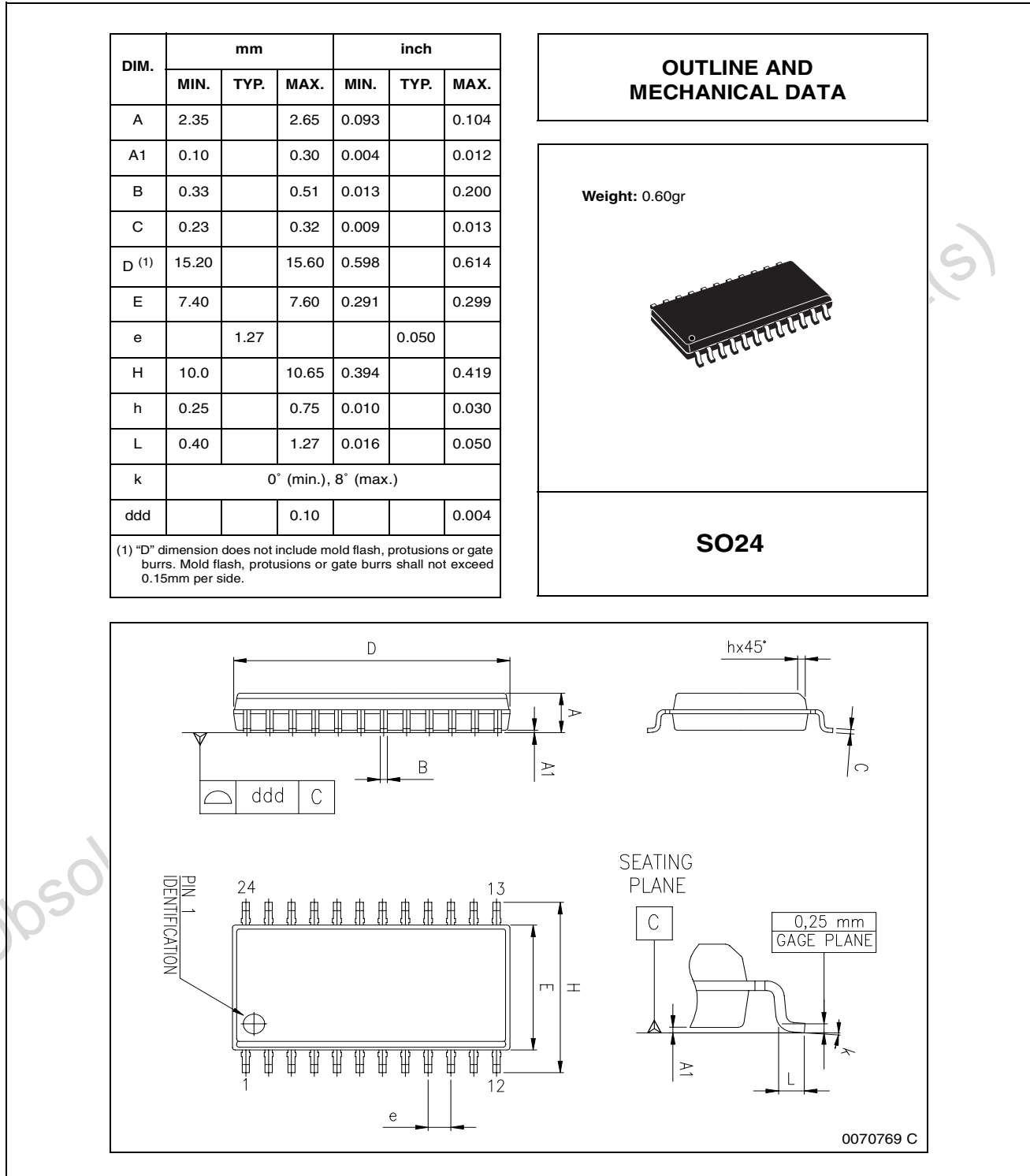
Figure 22. SO24 Mechanical Data & Package Dimensions
