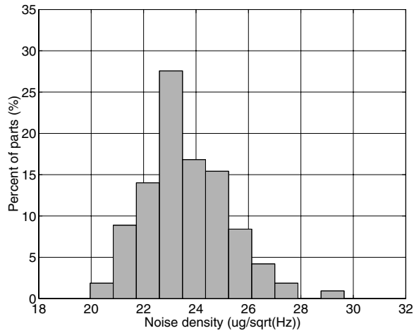
Figure 19. Noise density at 3.3V (Z axis)
