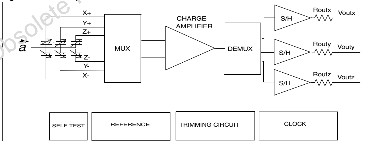
Figure 2. Block Diagram
