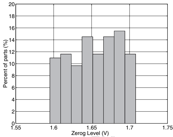
Figure 8. Z axis Zero g Level at 3.3V
