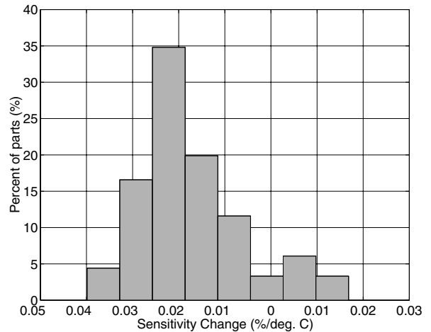
Figure 17. Z axis Sensitivity Change Vs. Temperature
