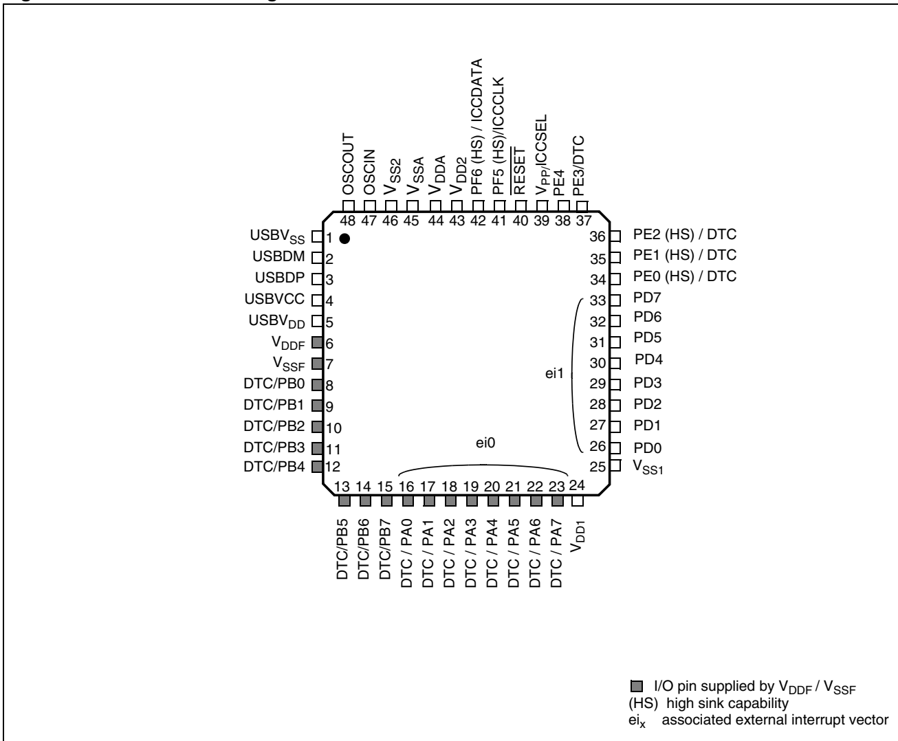
Figure 4. 48-Pin LQFP Package Pinout
