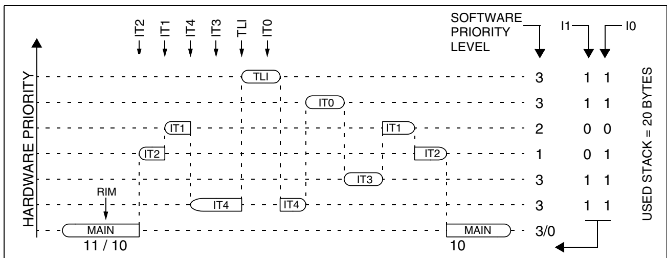
Figure 28. Nested Interrupt Management
