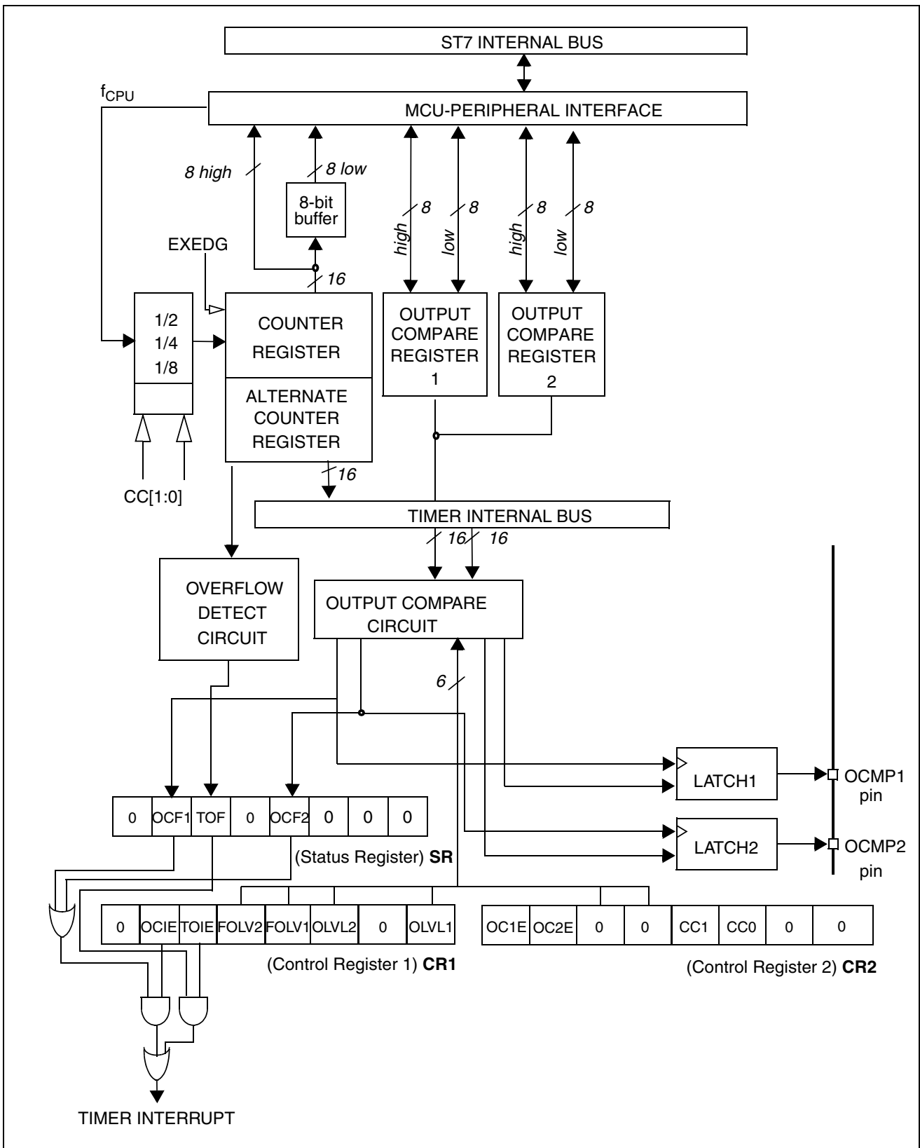
Figure 41. Timer Block Diagram
