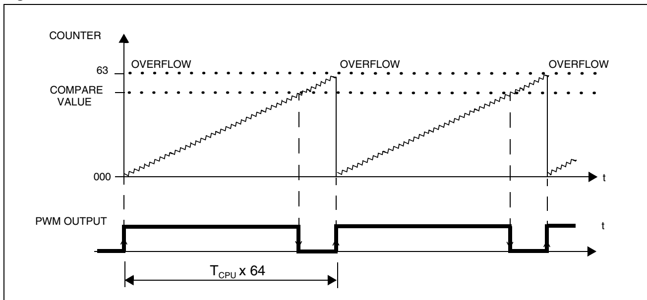
Figure 48. PWM Generation
