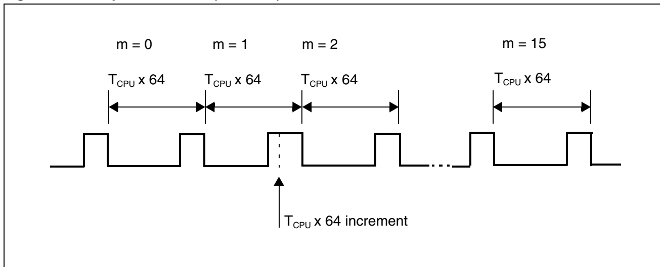
Figure 51. BRM pulse addition (PWM > 0)
