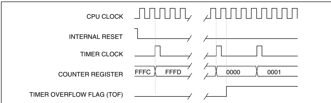
Figure 43. Counter Timing Diagram, internal clock divided by 4
