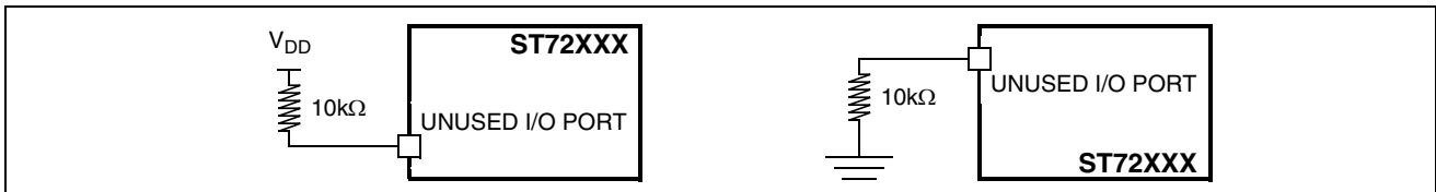
Figure 75 Two typical Applications with unused I/O Pin
