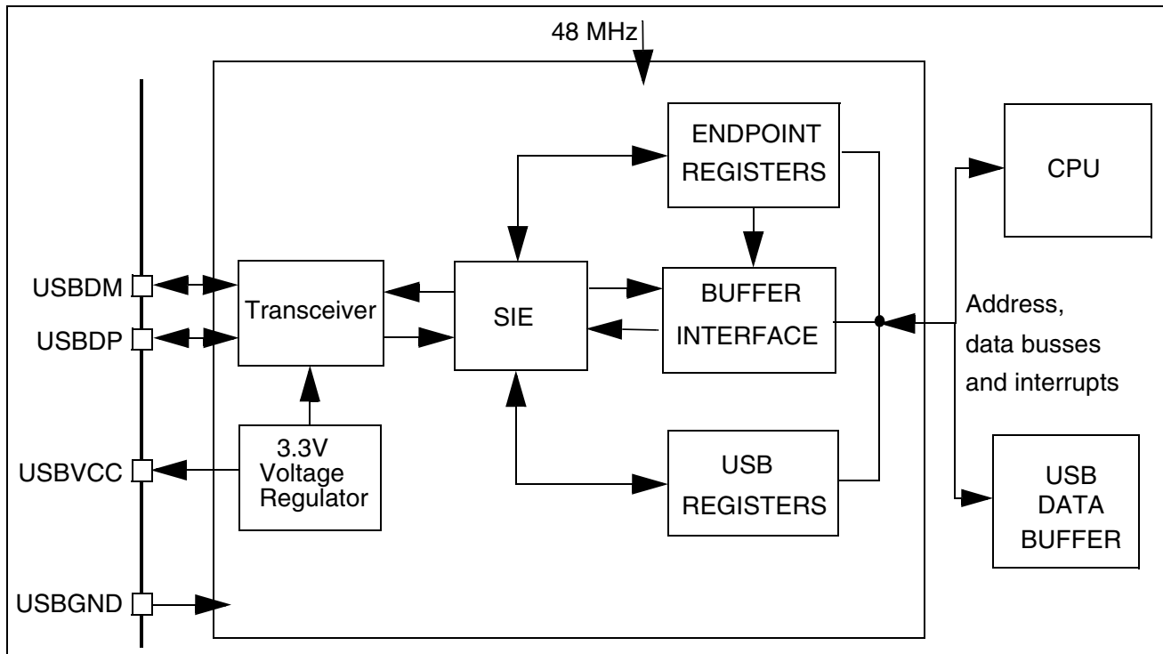
Figure 36. USB Block Diagram
