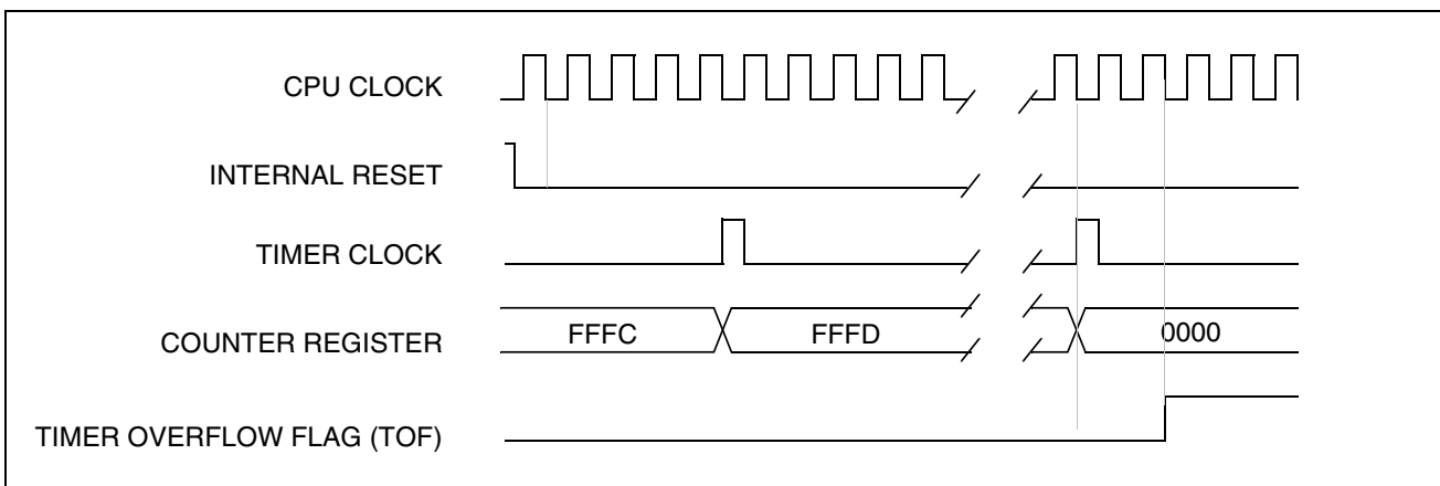
Figure 44. Counter Timing Diagram, internal clock divided by 8
