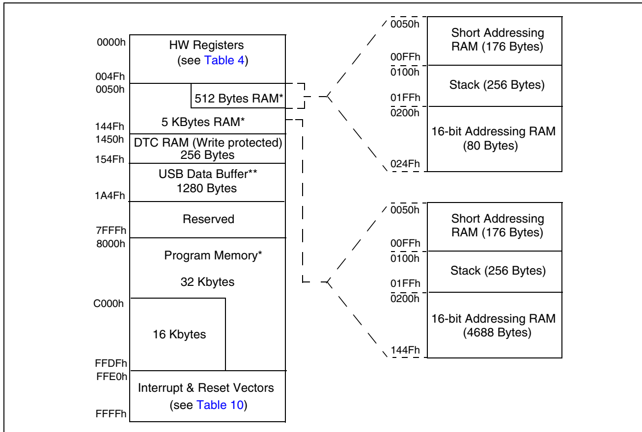
Figure 10. Memory Map
