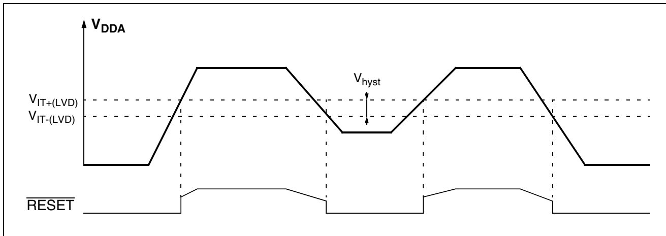
Figure 21. Low Voltage Detector vs Reset
