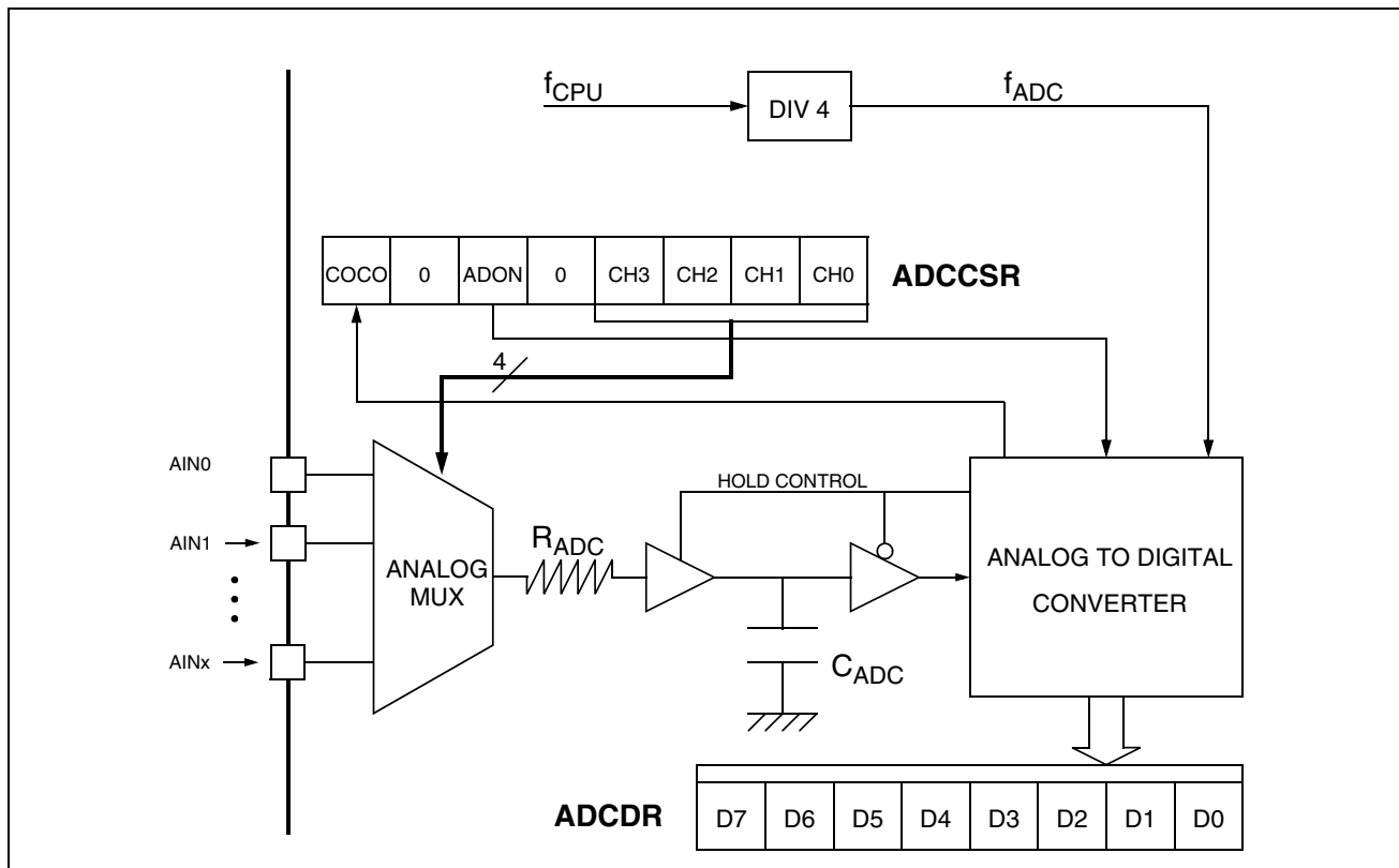
Figure 66. ADC Block Diagram
