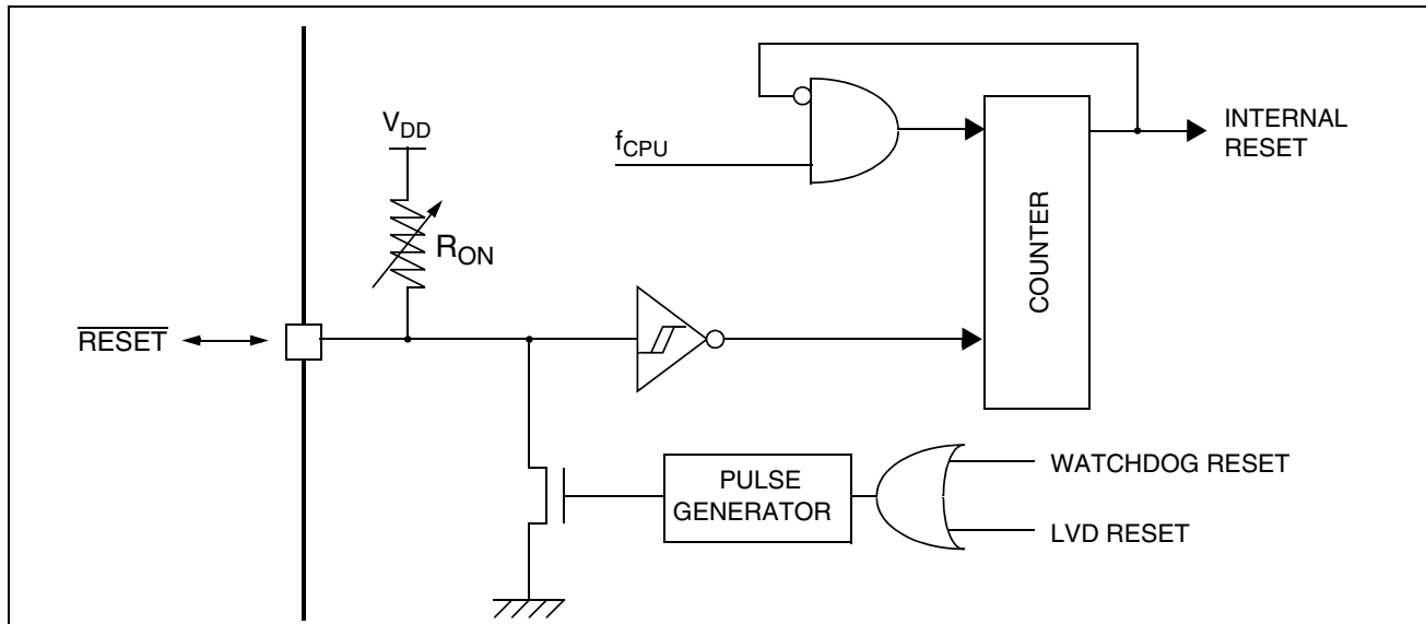
Figure 18. Reset Block Diagram
