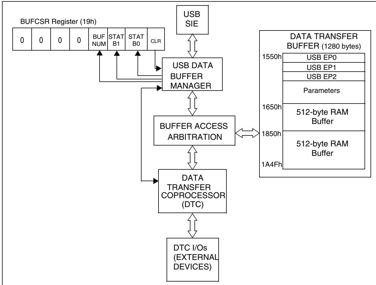
Figure 40. Overview of USB, DTC and ST7 Interconnections
