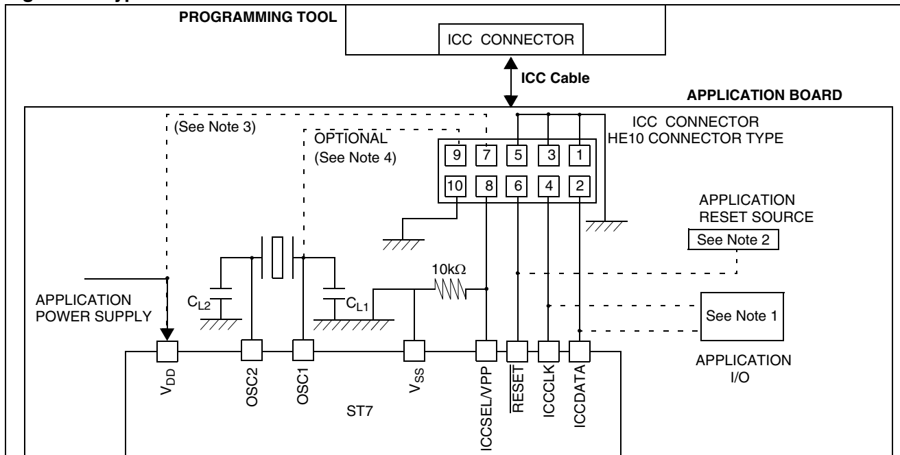
Figure 12. Typical ICC Interface
