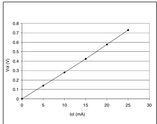
Figure 81. Typical V_{OL} at V_{DD}=5V (high-sink)
