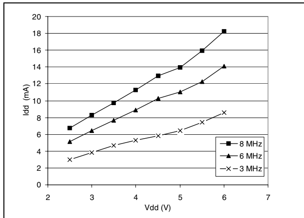
Figure 71. Typical I_{DD} in RUN vs. f_{CPU}
