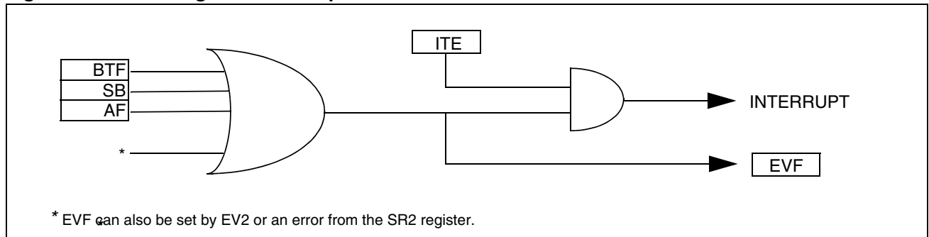
Figure 65. Event Flags and Interrupt Generation
