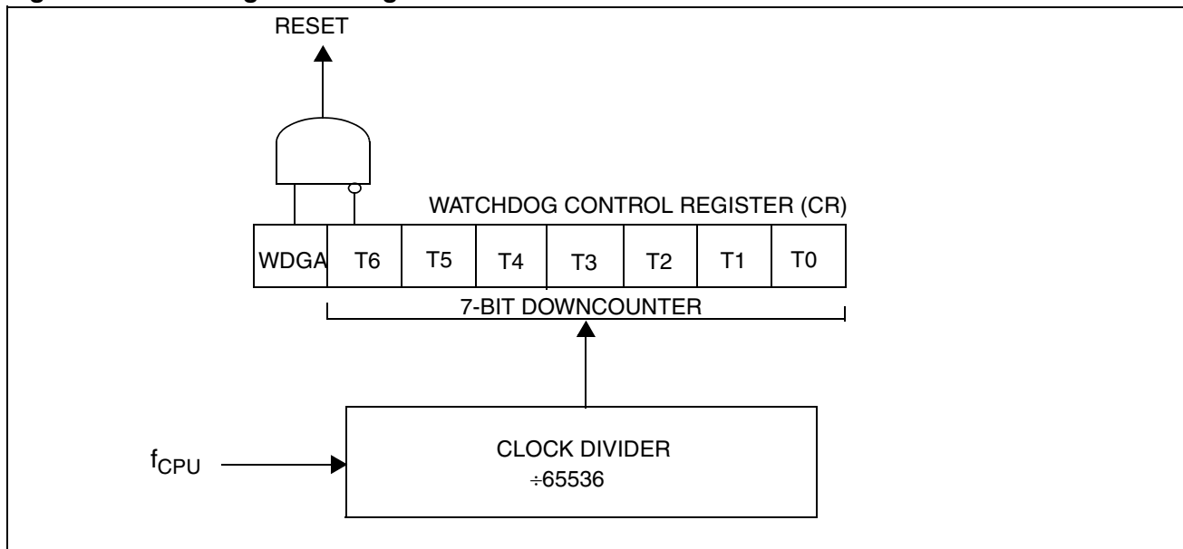
Figure 33. Watchdog Block Diagram
