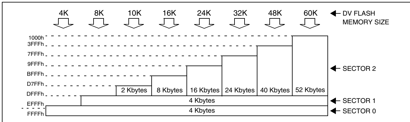
Figure 11. Memory Map and Sector Address
