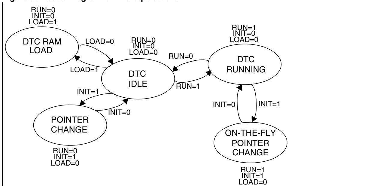
Figure 35. State Diagram of DTC Operations
