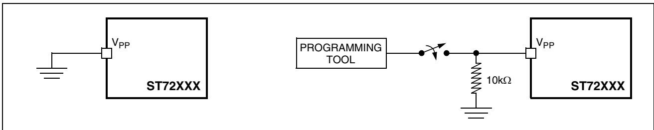
Figure 74. Two typical Applications with V_{PP} Pin 1)
