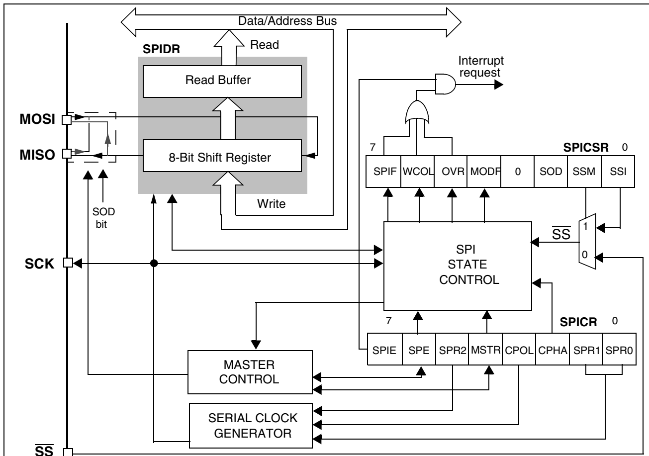
Figure 55. Serial Peripheral Interface Block Diagram
