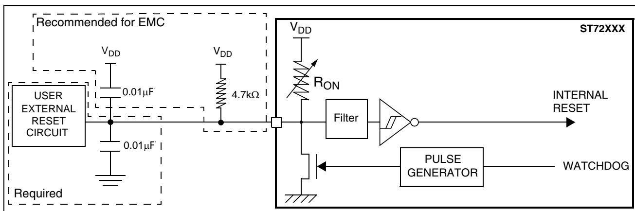
Figure 86. \overline{\text{RESET}} pin protection when LVD is disabled. 1)
