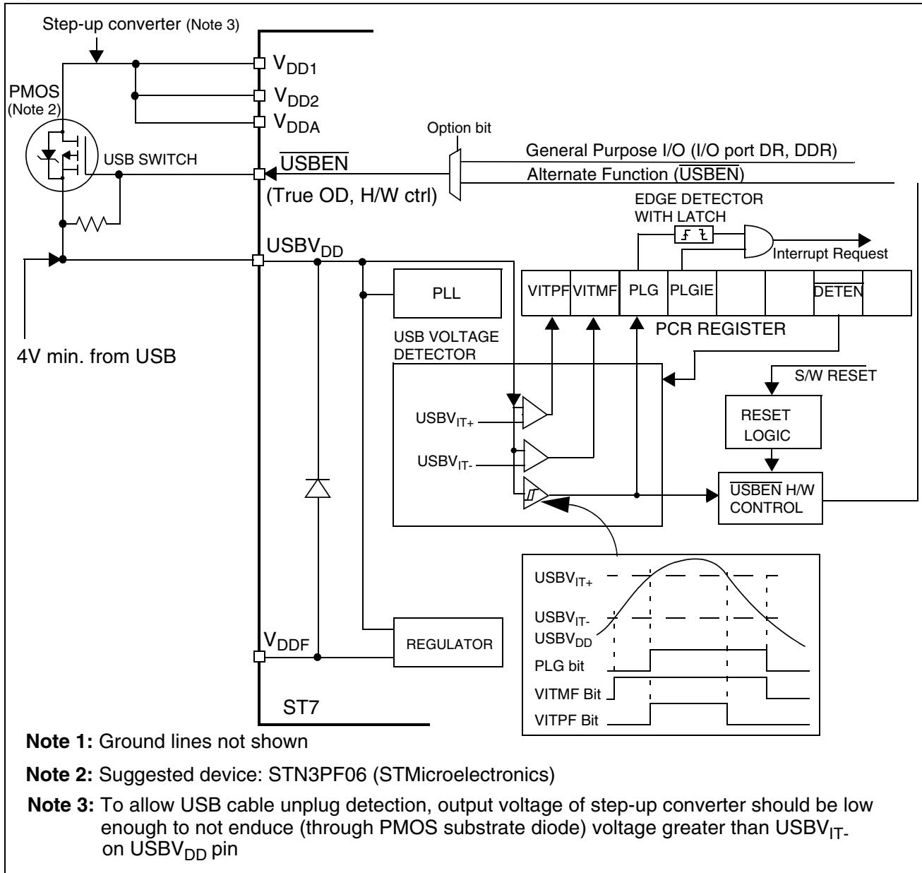
Figure 23. External Power Supply Switch
