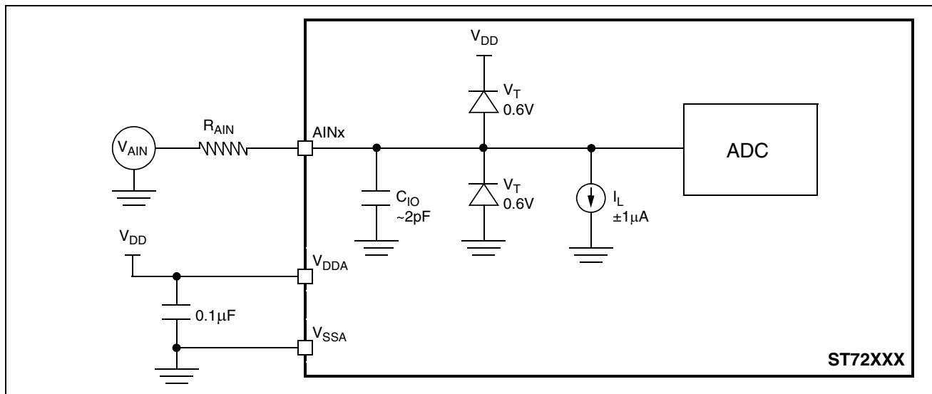
Figure 93. Typical Application with ADC
