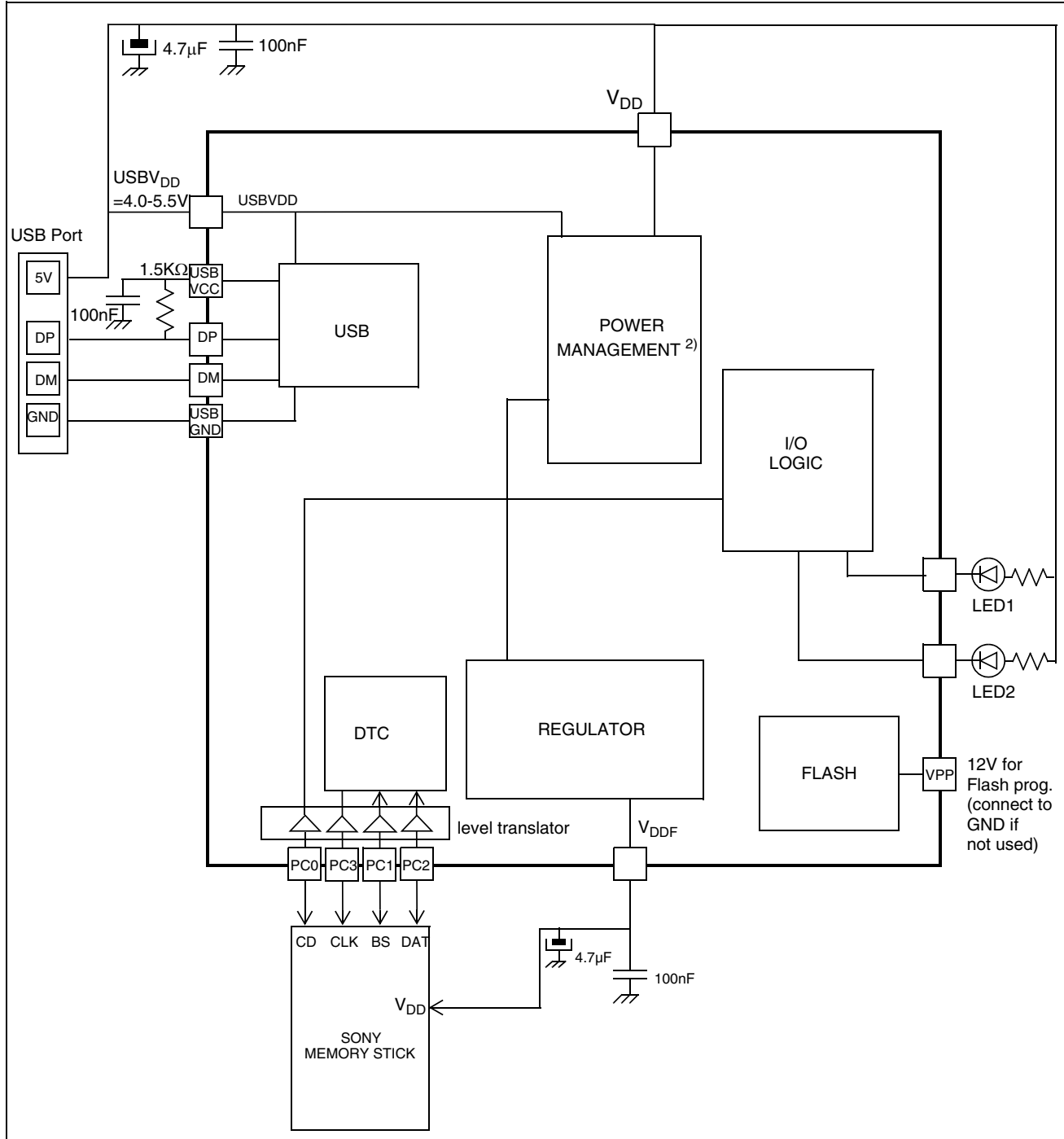
Figure 9. Sony Memory Stick Writer Application Example
