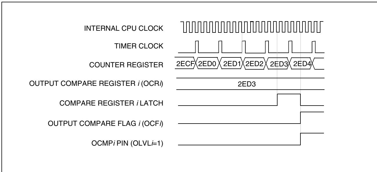
Figure 47. Output Compare Timing Diagram, f_{\text{TIMER}} = f_{\text{CPU}}/4
