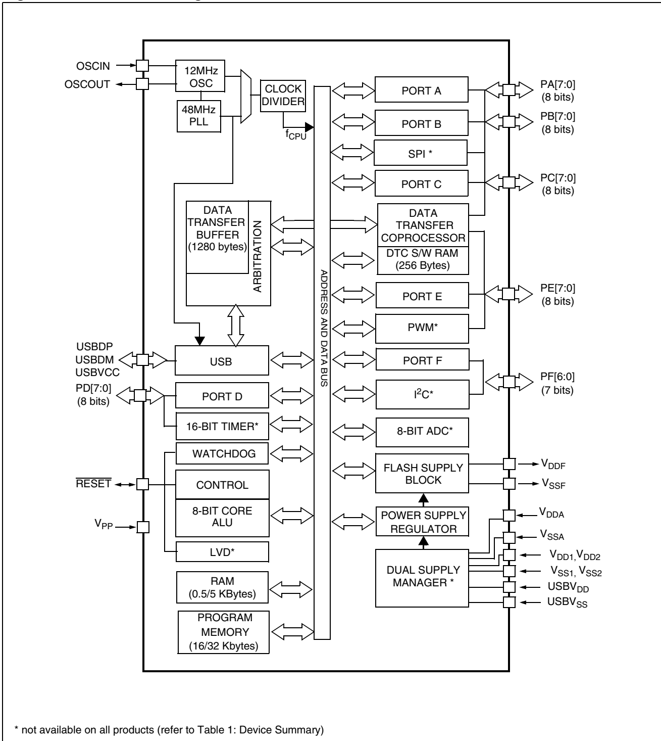
Figure 3. ST7265x Block Diagram
