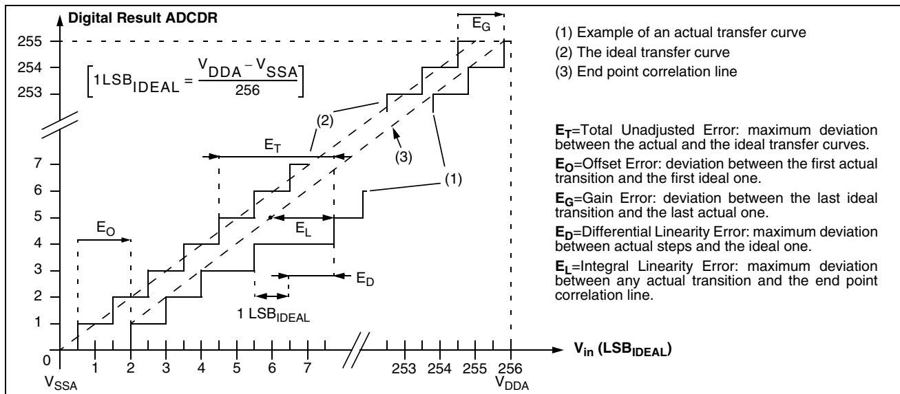
Figure 94. ADC Accuracy Characteristics
