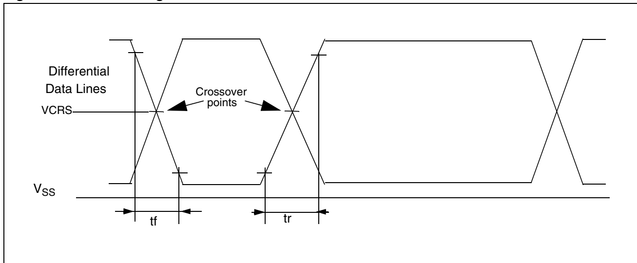
Figure 92. USB: Data Signal Rise and Fall Time
