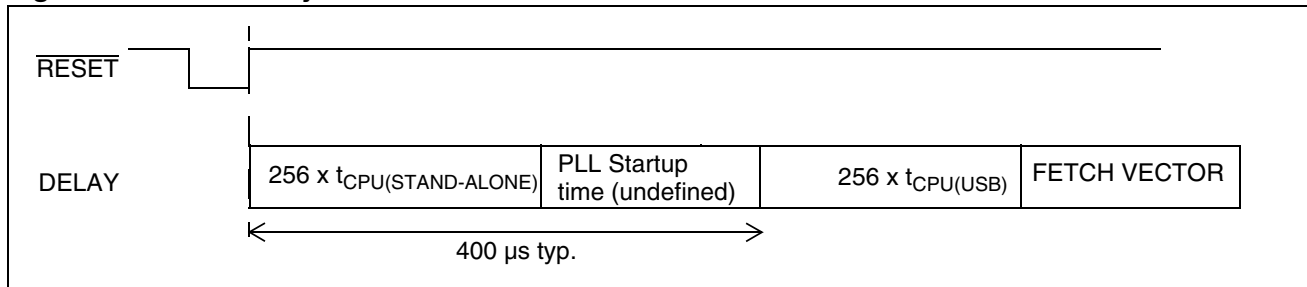
Figure 20. Reset Delay in USB Mode
