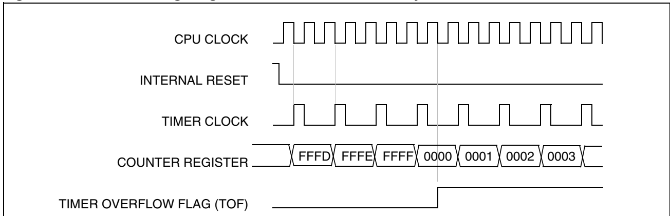
Figure 42. Counter Timing Diagram, internal clock divided by 2
