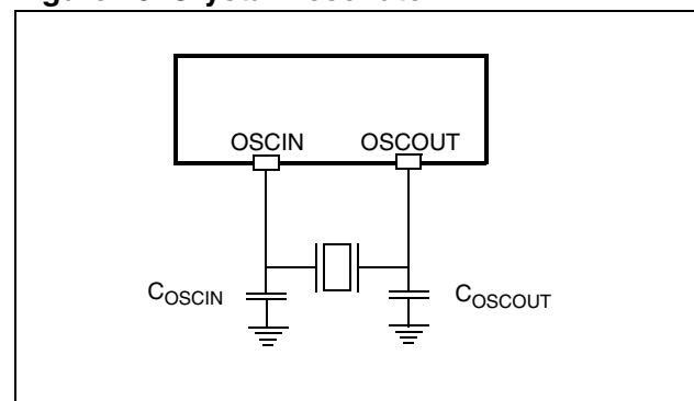
Figure 16. Crystal Resonator
