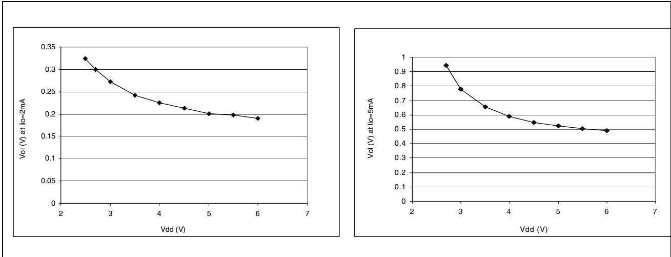
Figure 83. Typical V_{OL} vs. V_{DD} (high-sink I/Os)
