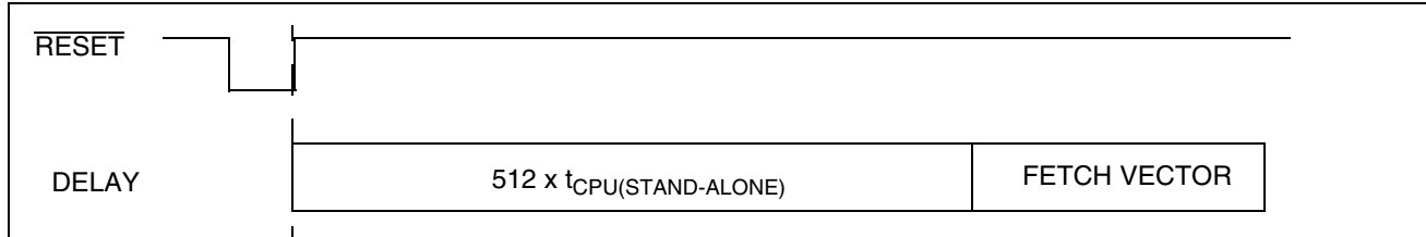
Figure 20. Reset Delay in USB Mode
