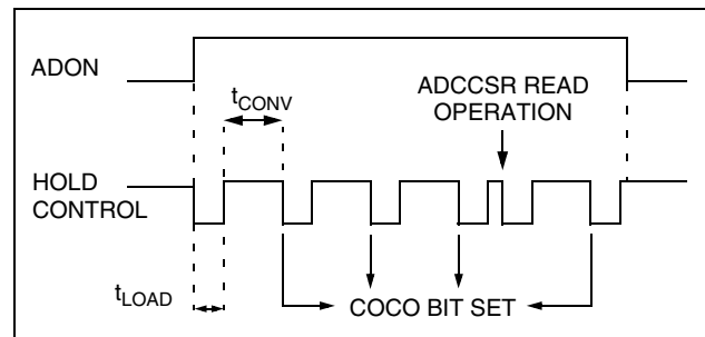
Figure 67. ADC Conversion Timings
