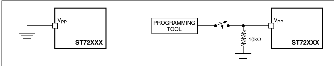
Figure 87. Two typical Applications with V PP Pin 2)
