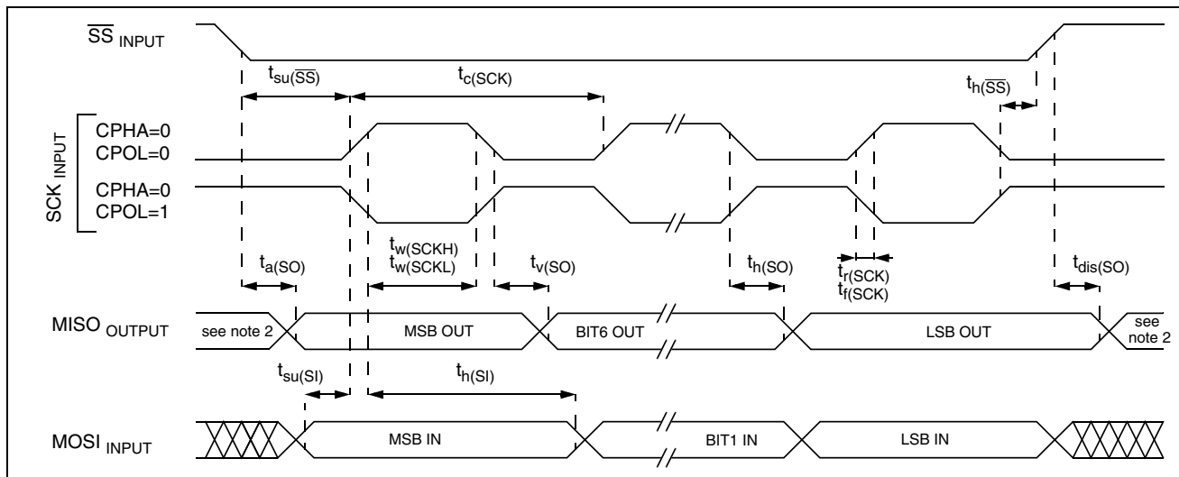
Figure 88. SPI Slave Timing Diagram with CPHA=0 3)
