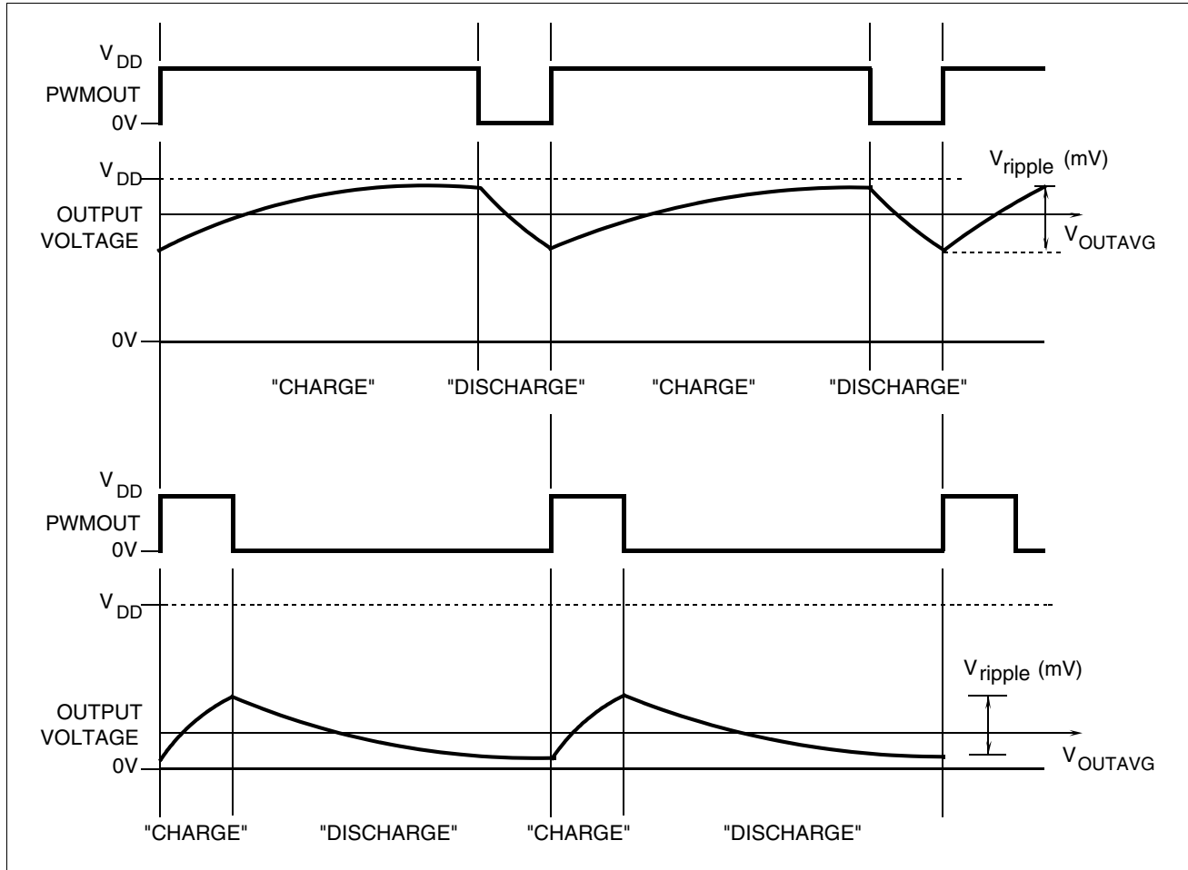
Figure 50. PWM Simplified Voltage Output After Filtering
