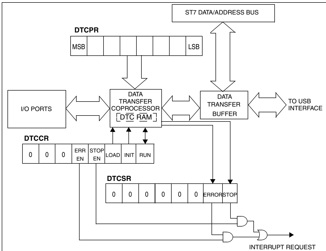
Figure 34. DTC Block Diagram
