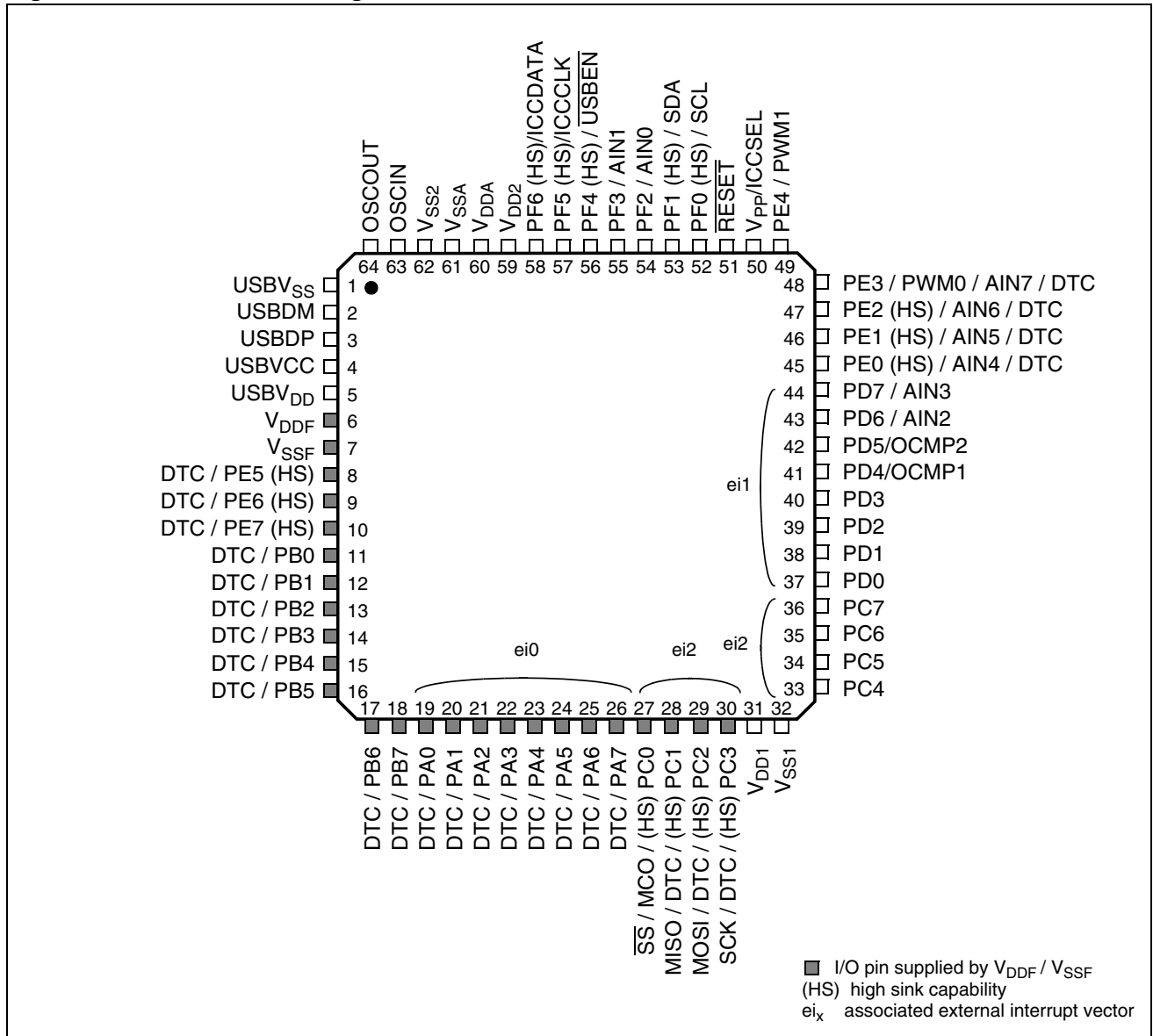
Figure 5. 64-Pin LQFP Package Pinout
