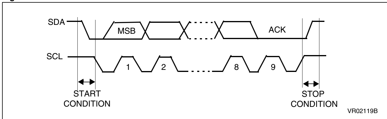
Figure 62. I 2 C BUS Protocol
