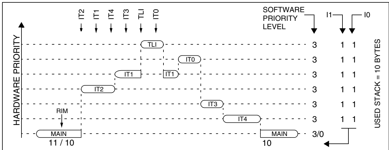
Figure 27. Concurrent Interrupt Management
