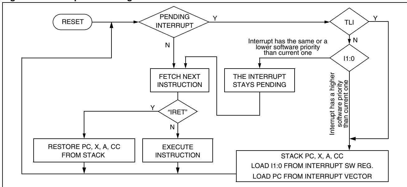
Figure 25. Interrupt Processing Flowchart
