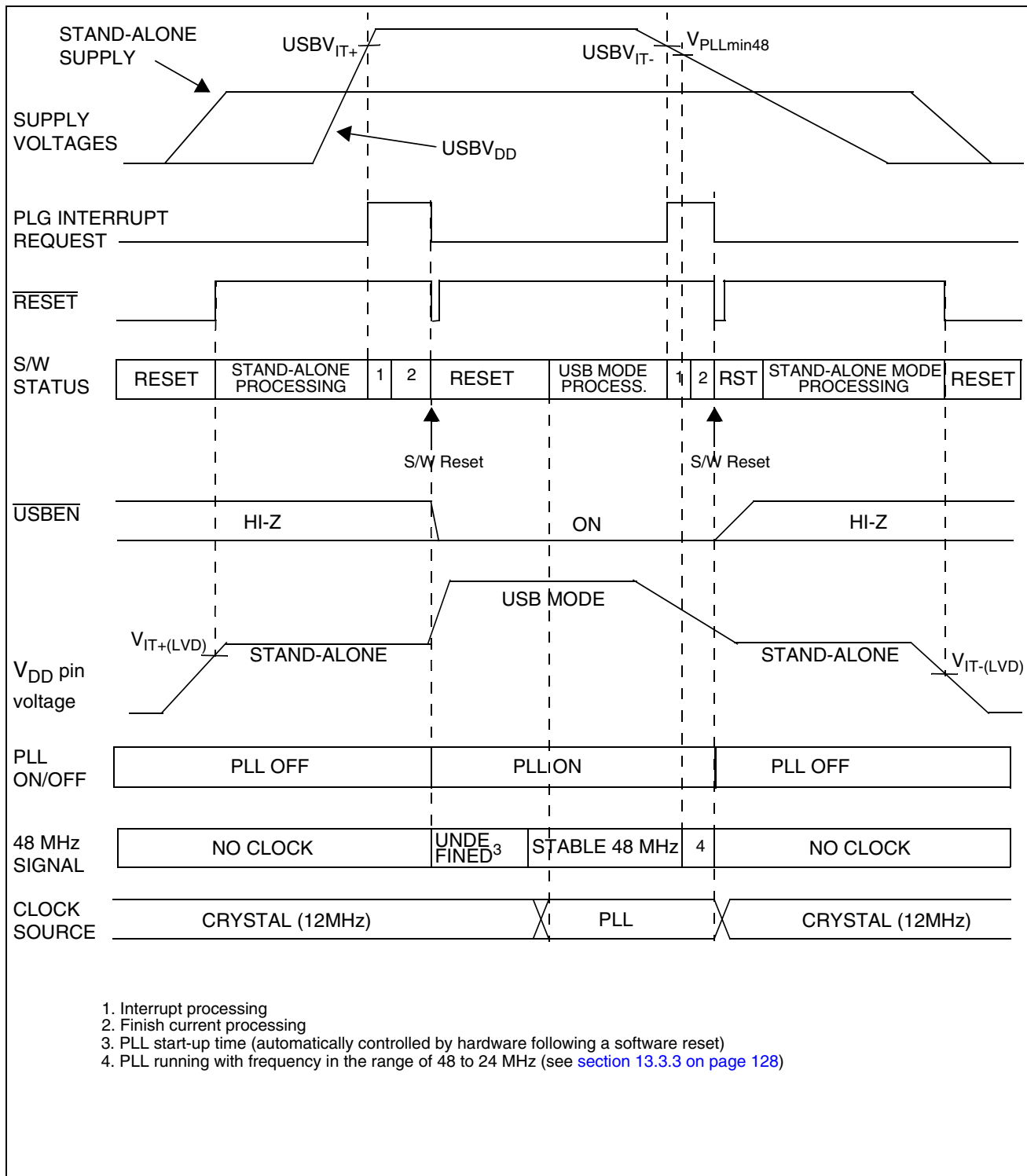
Figure 24. Power Supply Management: Dual Power Supply
