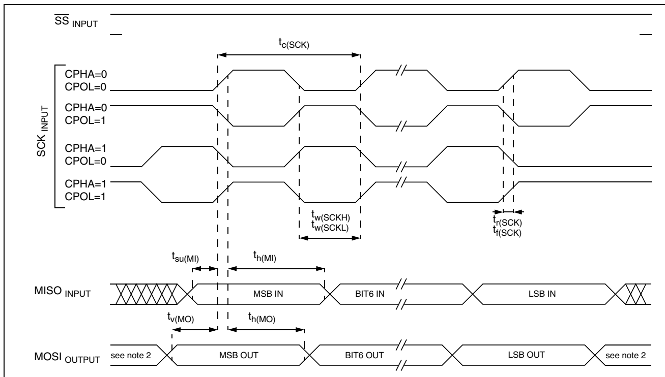
Figure 90. SPI Master Timing Diagram 1)
