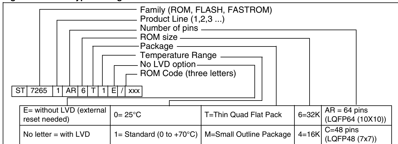
Figure 97. Sales Type Coding Rules 2)
