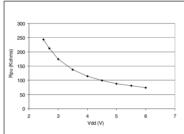
Figure 78. Typical R_{PU} vs. V_{DD} with V_{IN}=V_{SS}
