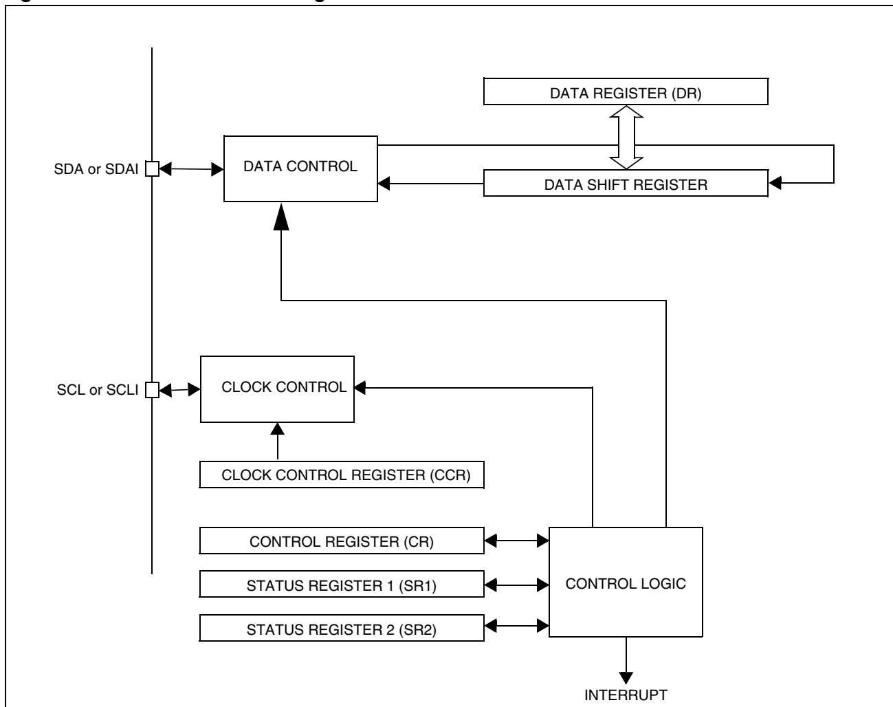
Figure 63. I 2 C Interface Block Diagram
