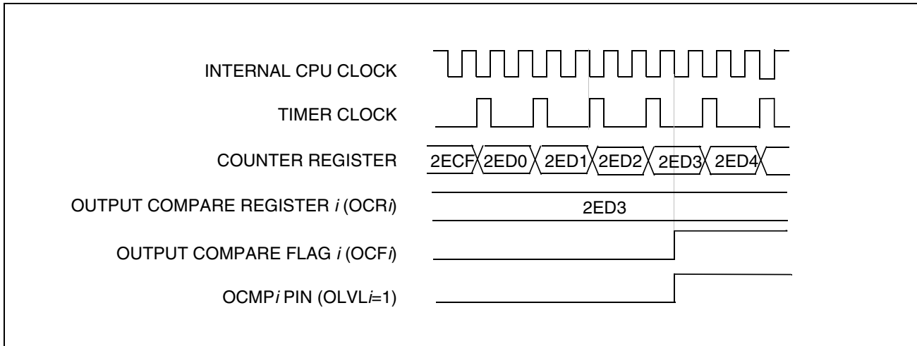
Figure 46. Output Compare Timing Diagram, f_{\text{TIMER}} = f_{\text{CPU}}/2
