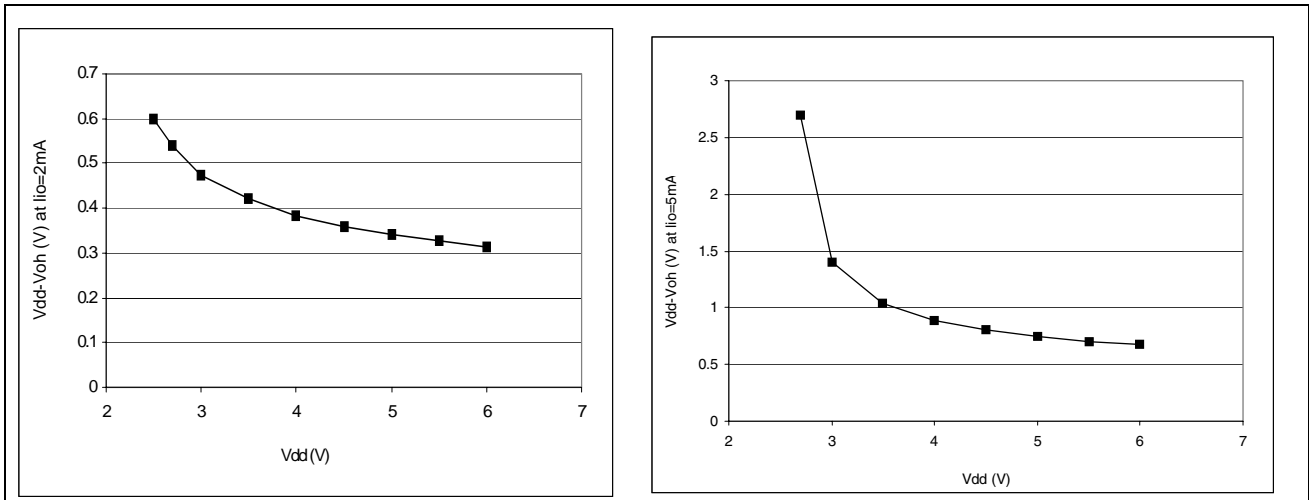
Figure 84. Typical V_{OH} vs. V_{DD}
