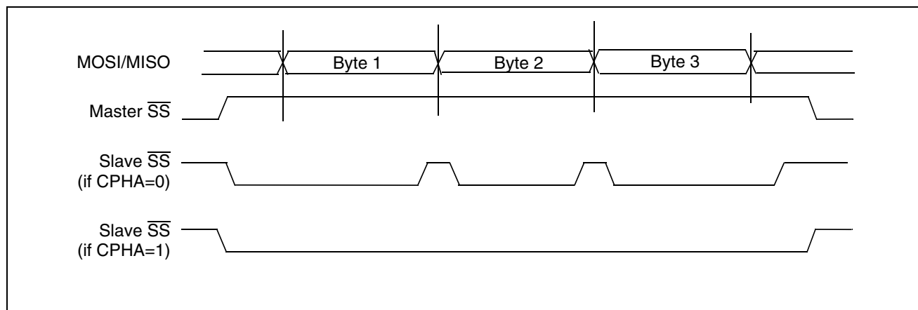
Figure 58. Hardware/Software Slave Select Management
