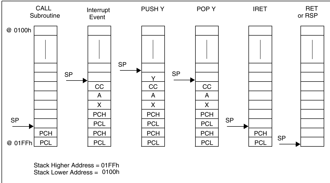
Figure 14. Stack Manipulation Example
