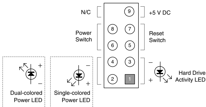
Figure 24. Connection Diagram for Front Panel Connector
