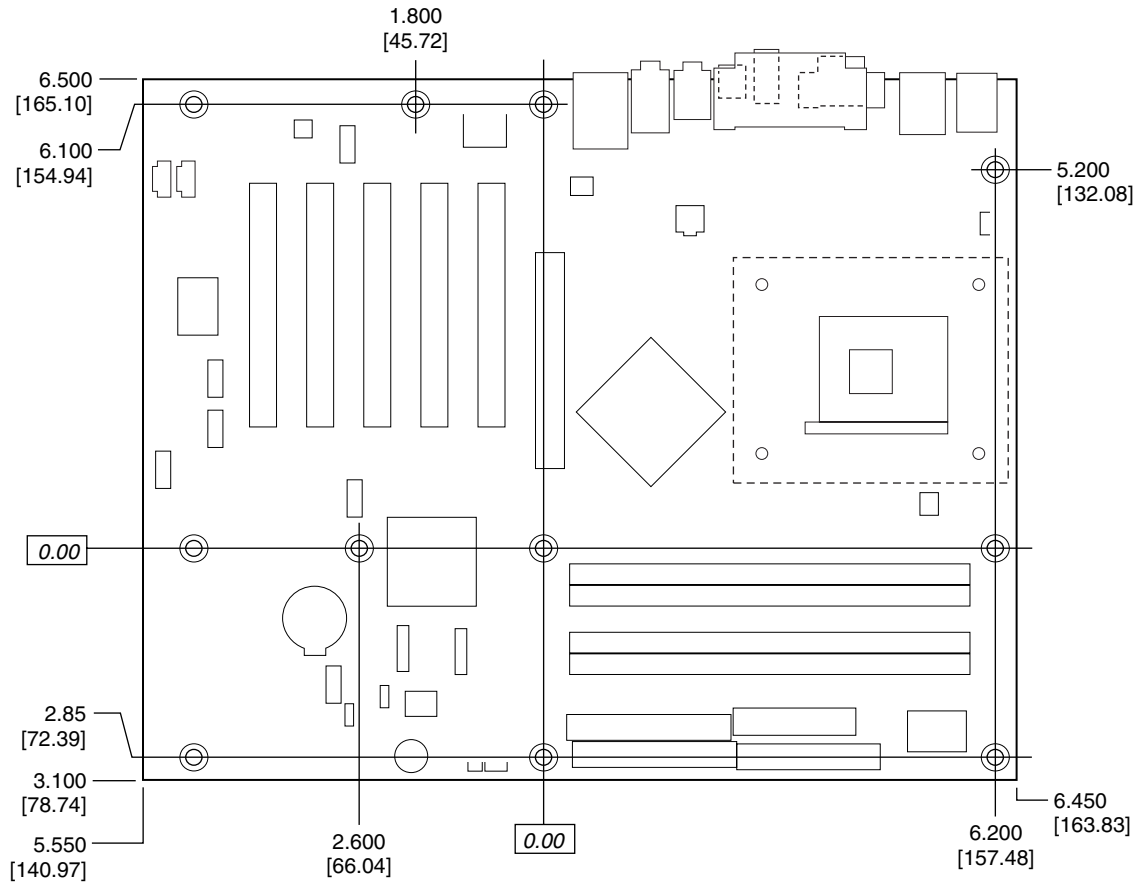
Figure 28. Board Dimensions
