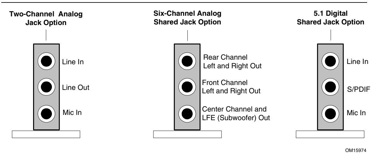
Figure 11. Back Panel Audio Connector Options for Flex 6 Audio Subsystem
