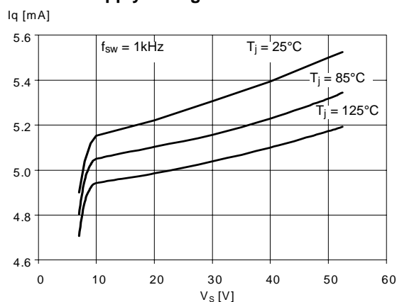
Figure 21. Typical Quiescent Current vs. Supply Voltage
