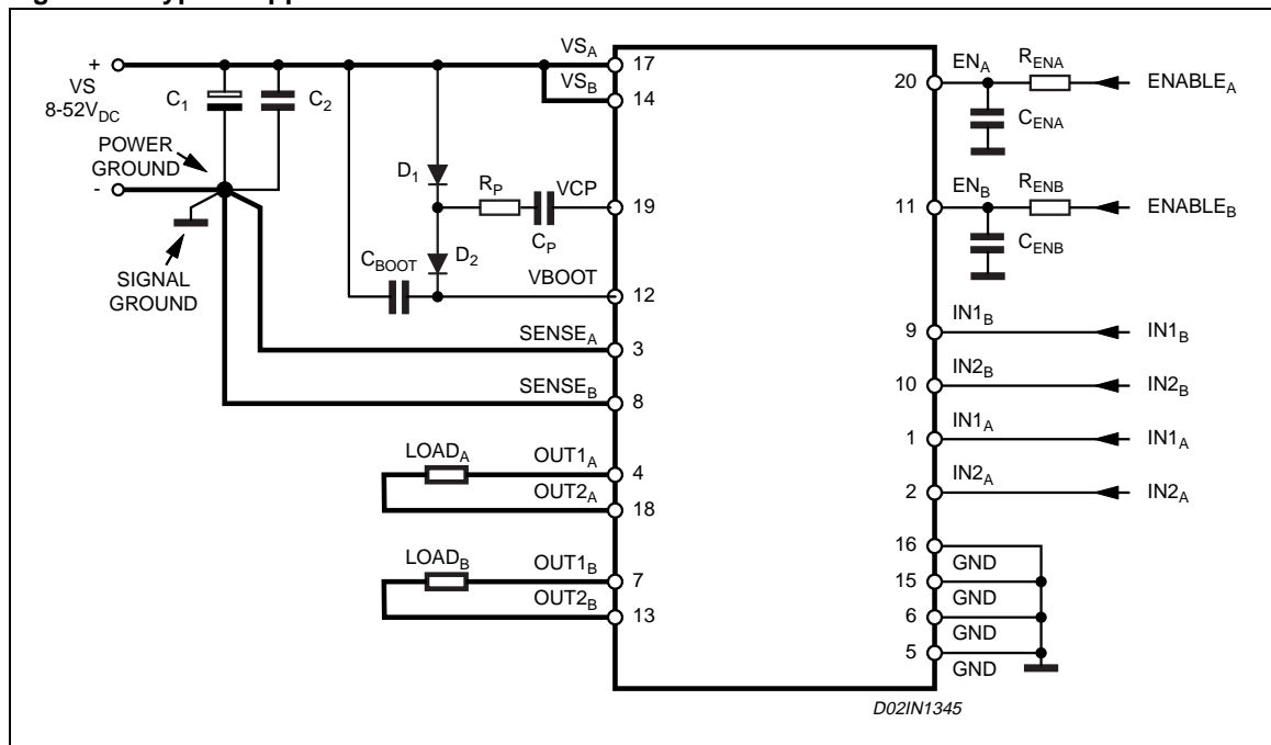
Figure 11. Typical Application
