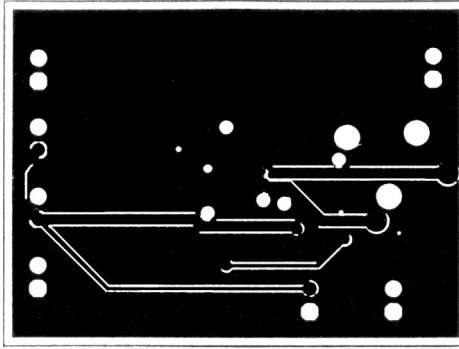
FIGURE 15. Recommended LD PC Board Layout: Upper Inner-Layer Layout
