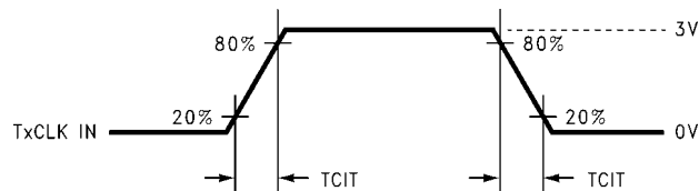
FIGURE 4. DS90CR483A (Transmitter) Input Clock Transition Time
