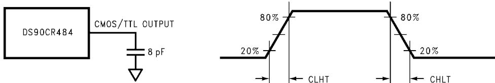
FIGURE 3. DS90CR484A (Receiver) CMOS/TTL Output Load and Transition Times
