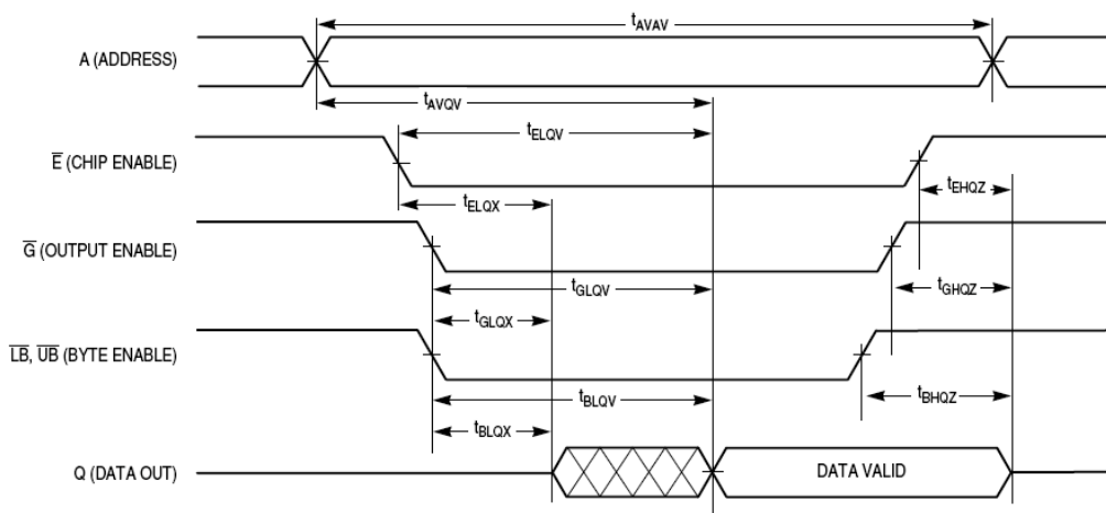
Figure 5. Read Cycle 2
