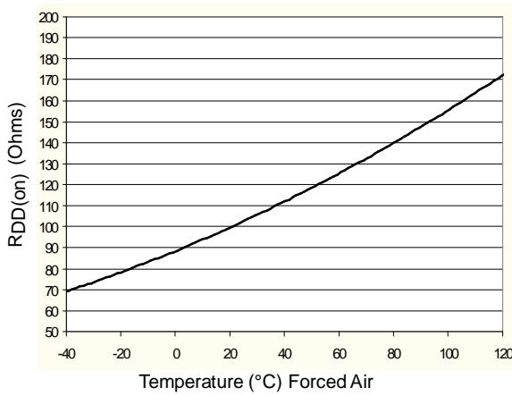
Figure 3. Typical On-Resistance
