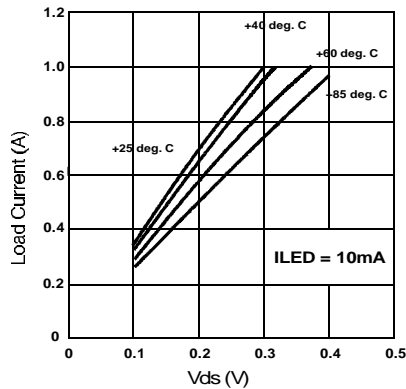
Figure 3. Typical On-Characteristics
