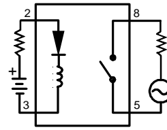
Electromechanical Analogy
