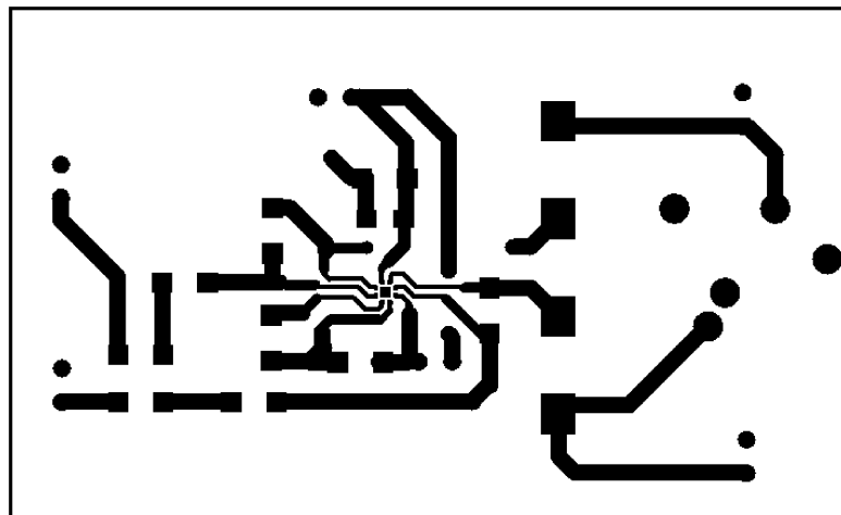
FIGURE 10. Recommended LQ PC Board Layout Component-Side Layout
