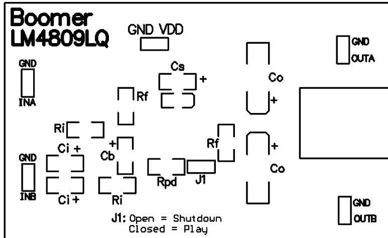
FIGURE 9. Recommended LQ PC Board Layout Component-Side Silkscreen
