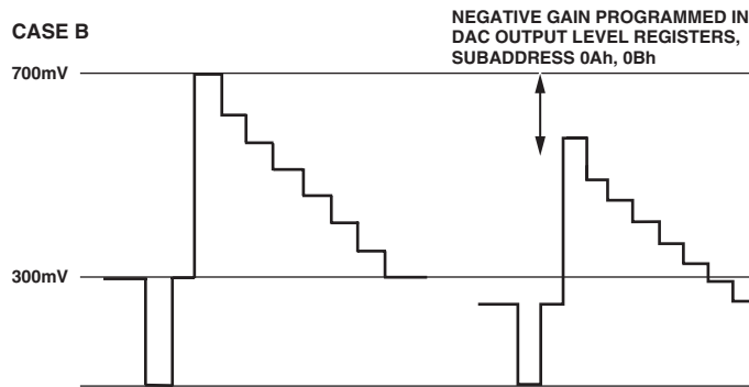
Figure 40. Programmable DAC Gain—Positive and Negative Gain
