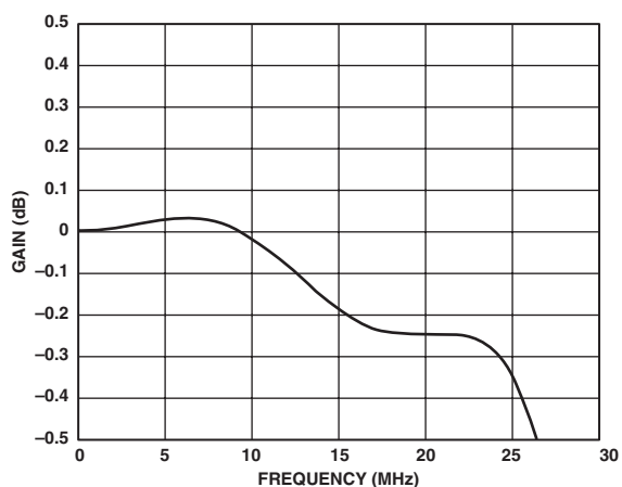
Figure 37. HD Sinc Filter Disabled
