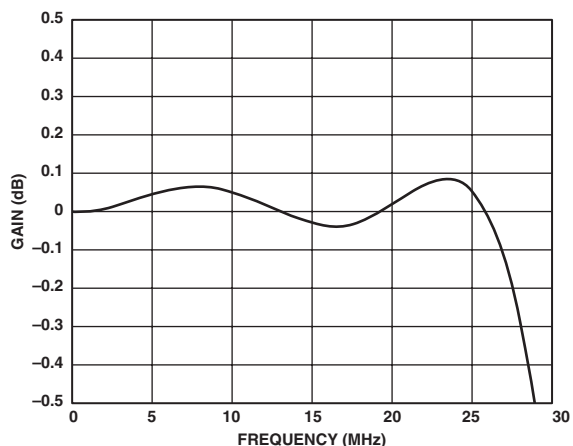
Figure 36. HD Sinc Filter Enabled
