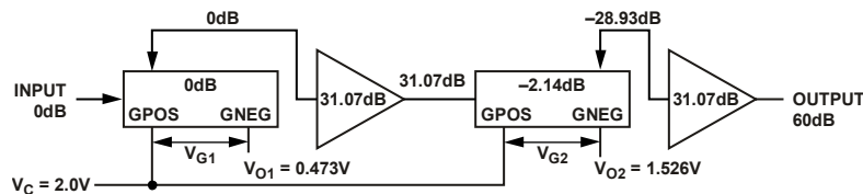
Figure 38. AD603 Gain Control Input Calculations for Sequential Operation V_c = 2.0 V
