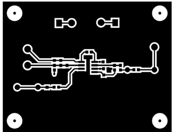
Figure 50. Component Side Copper
