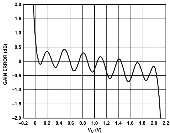
Figure 43. Gain Error for Cascaded Stages—Parallel Control
