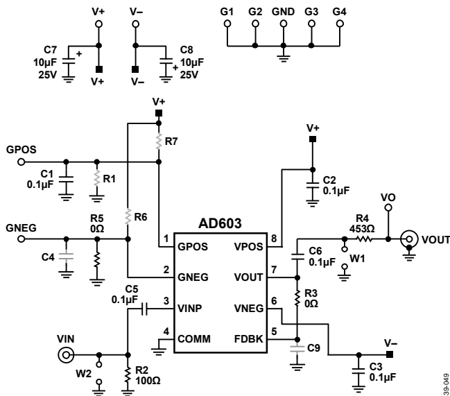
Figure 49. Schematic of the AD603 Evaluation Board
