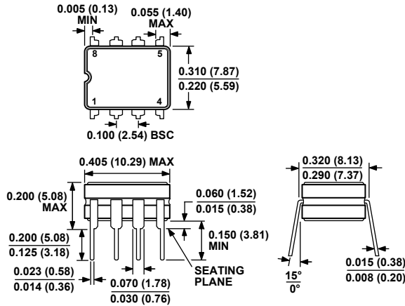
Figure 53. 8-Lead Ceramic Dual In-Line Package [CERDIP] (Q-8)
