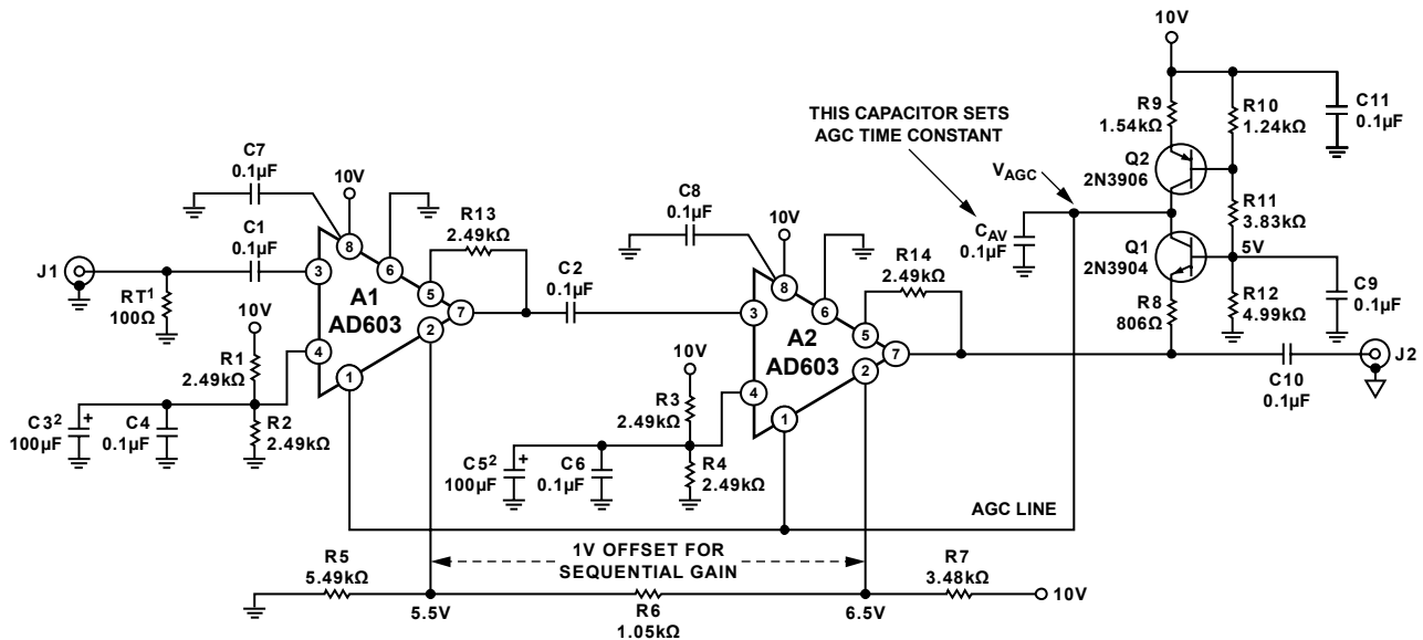
Figure 47. A Low Noise AGC Amplifier
