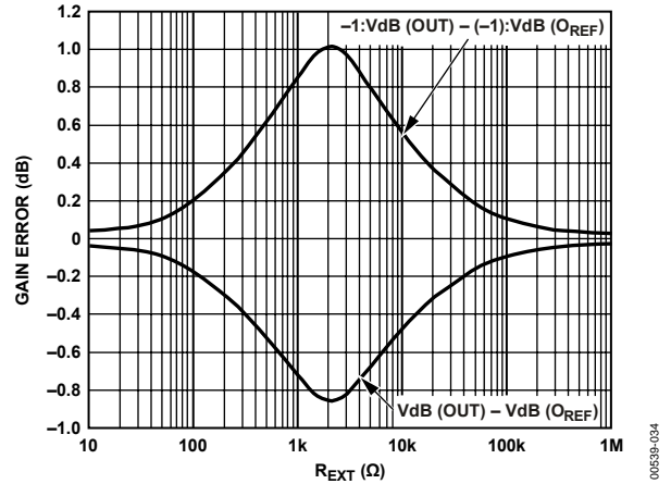
Figure 34. Worst-Case Gain Error, Assuming Internal Resistors Have a Maximum Tolerance of -20\% (Top Curve) or +20\% (Bottom Curve)
