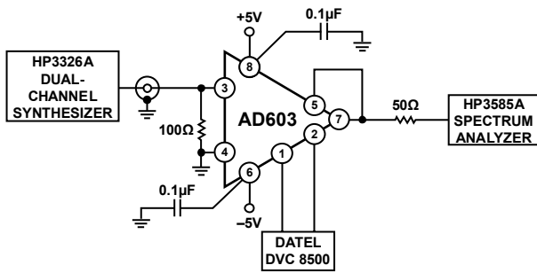
Figure 23. Test Setup Used for: Noise Figure, Third-Order Intercept, and 1 dB Compression Point Measurements
