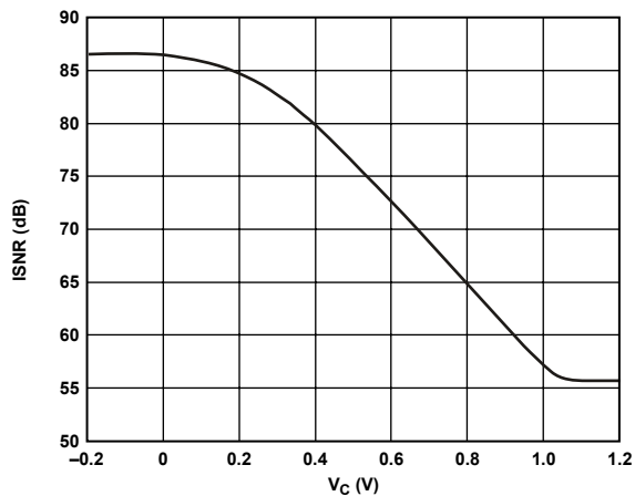
Figure 44. ISNR for Cascaded Stages—Parallel Control
