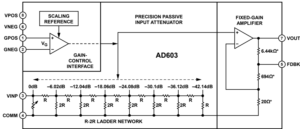
Figure 29. Simplified Block Diagram
