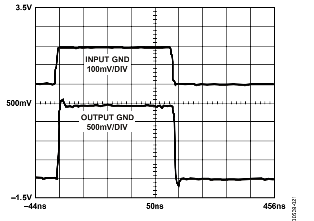
Figure 21. Transient Response, G = 20 dB (Input Is 500 ns Period, 50% Duty-Cycle Square Wave, Output Is Captured Using Tektronix 11402 Digitizing Oscilloscope)
