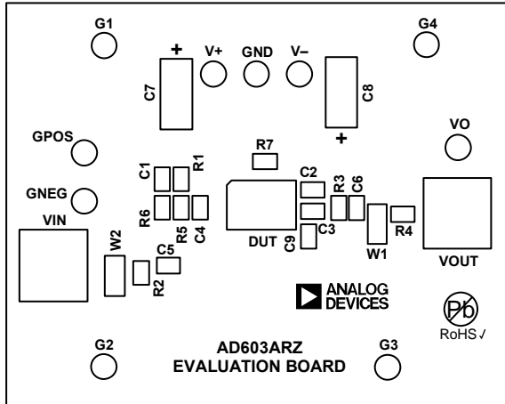
Figure 52. Component Side Silk Screen
