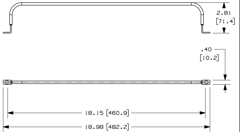
FIGURE 3 STRAIN RELIEF BAR
