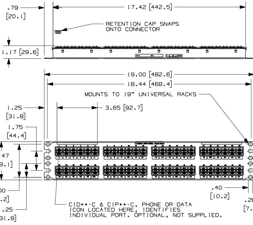
FIGURE 1 DP6 PLUS 48 PORT PATCH PANEL
