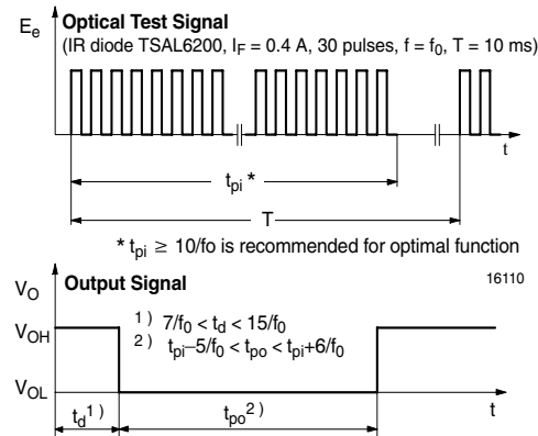
Figure 1. Output Function
