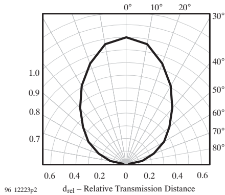
Figure 13. Directivity
