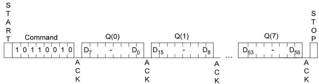
Figure 10. Initiatize Authentication
