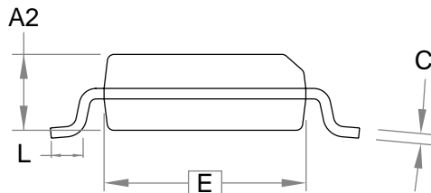
End View
