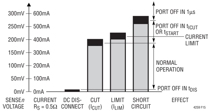
Figure 15. LTC4259 Current Sense and Limits
