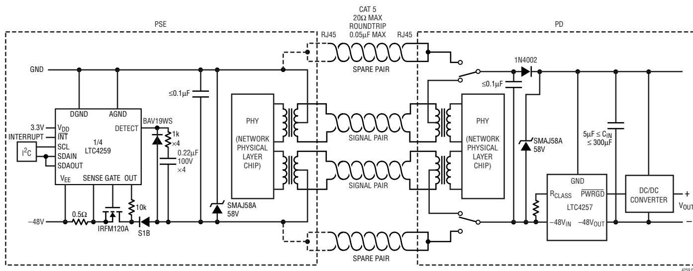
Figure 11. System Diagram
