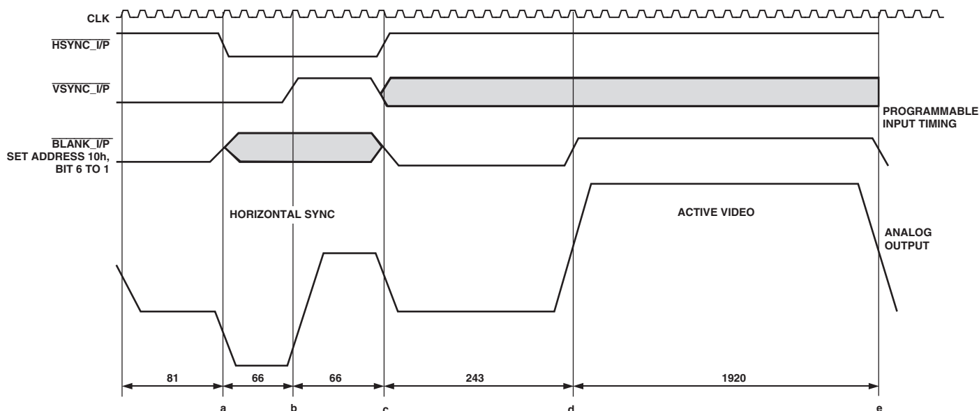
Figure 20a. Async Timing Mode—Programming Input Control Signals for SMPT 295M Compatibility
