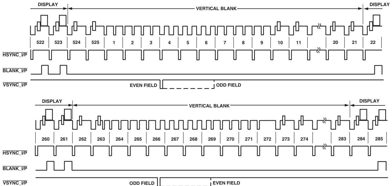
Figure 76. SD Slave Mode 2 (NTSC)
