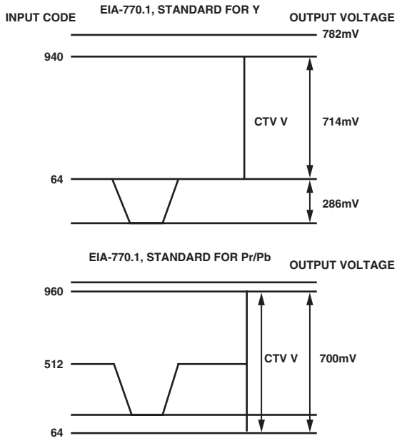
Figure 84. EIA 770.1 Standard Output Signals (525p/625p)
