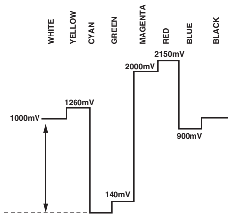
Figure 93. U Levels—NTSC
