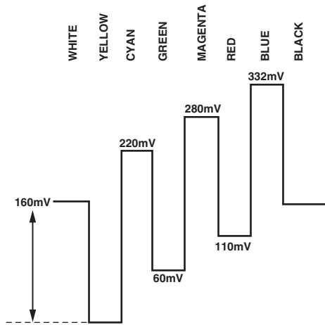
Figure 91. U Levels—NTSC
