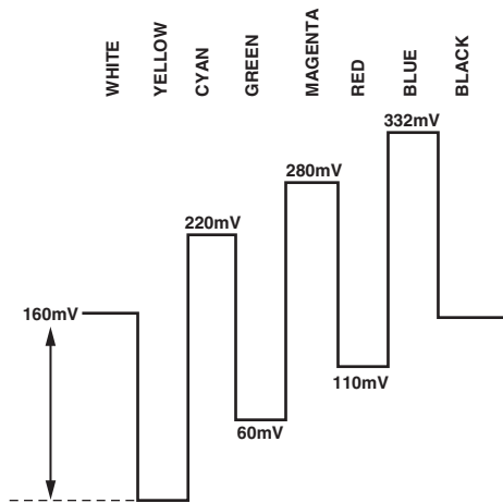
Figure 92. U Levels—PAL
