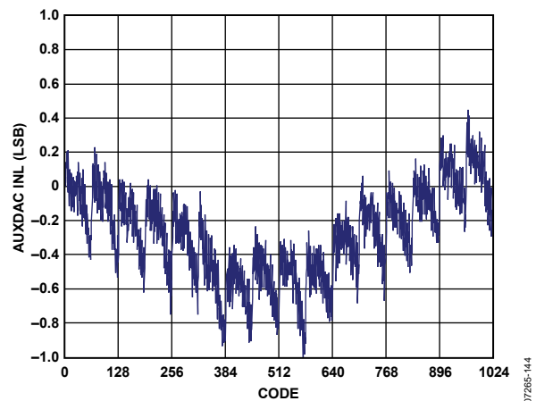
Figure 82. AUXDAC INL
