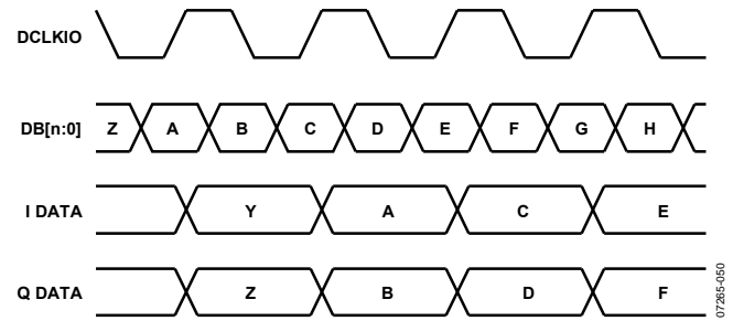
Figure 92. Timing Diagram with IFIRST = 1, IRISING = 1
