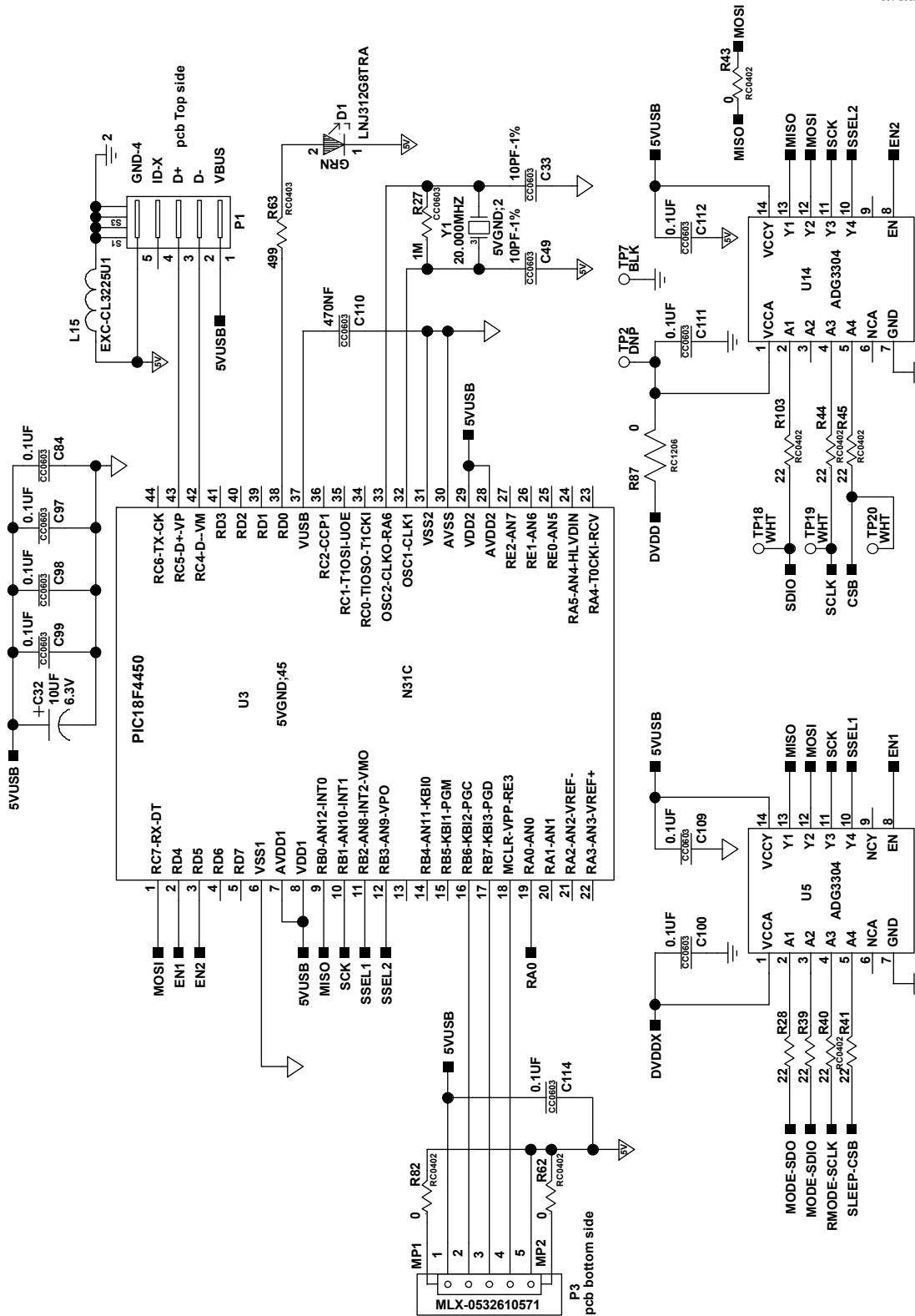
Figure 117. SPI Port
