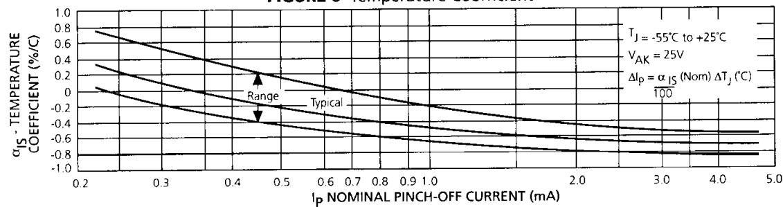
FIGURE 6 Temperature Coefficient
