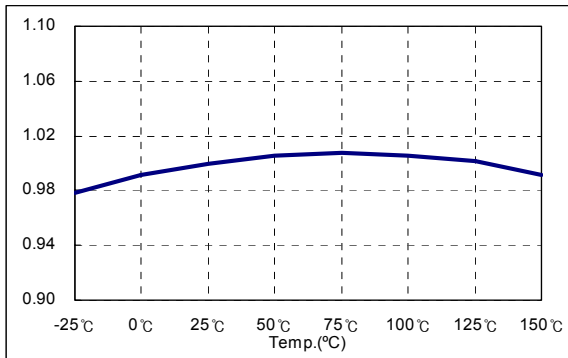
Figure 19. Peak Current Limit
