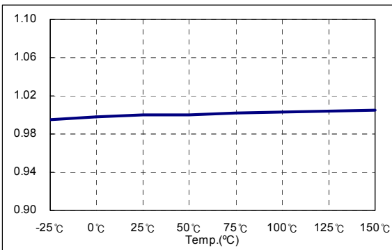
Figure 17. Primary Voltage
