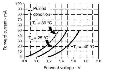
Fig. 1 IRED Forward Bias Characteristics
