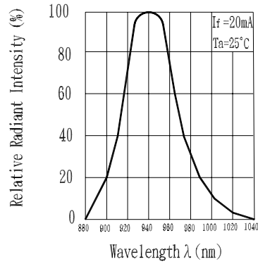
Fig. 2 Spectral Distribution
