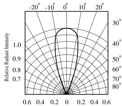
Fig. 6 Relative Radiant Intensity vs. Angular Displacement
