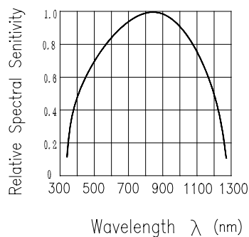
Fig.5 Spectral Sensitivity
