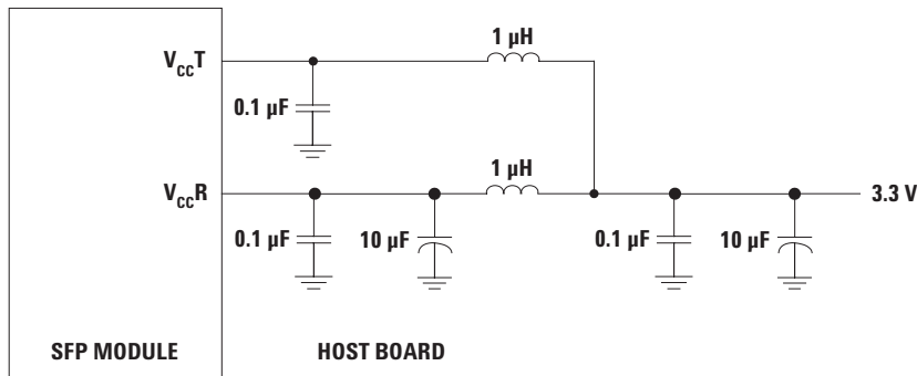
Figure 6. MSA required power supply filter
