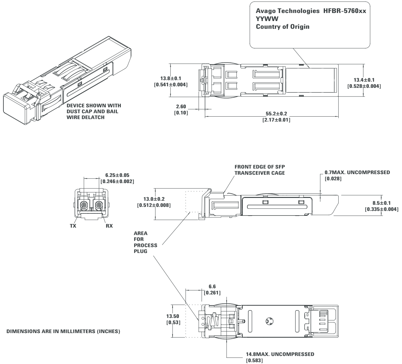
Figure 7a. Module drawing
