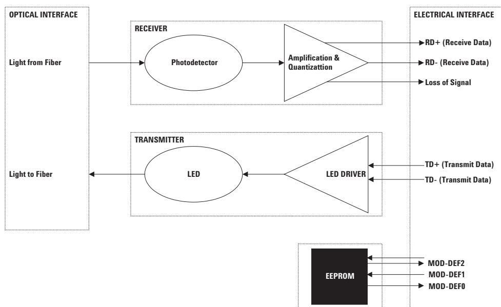
Figure 1. Transceiver functional diagram
